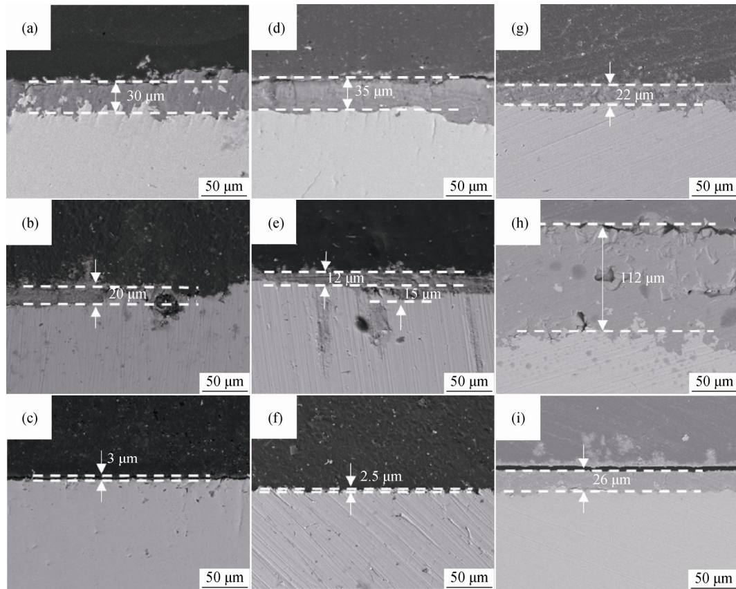
Fig. 11. Cross-sectional morphologies of the corrosion products: (a–c) No. 5; (d–f) No. 6; (g–i) No. 7. The first, second, and third lines represent X52, 3Cr, and 13Cr, respectively.
