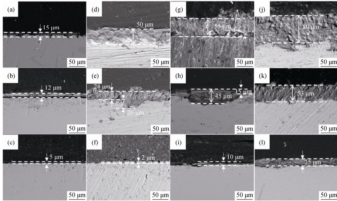
Fig. 6. Cross-sectional morphologies of the corrosion products: (a–c) No. 1; (d–f) No. 2; (g–i) No. 3; (j–l) No. 4. The first, second, and third lines represent X52, 3Cr, and 13Cr, respectively.
