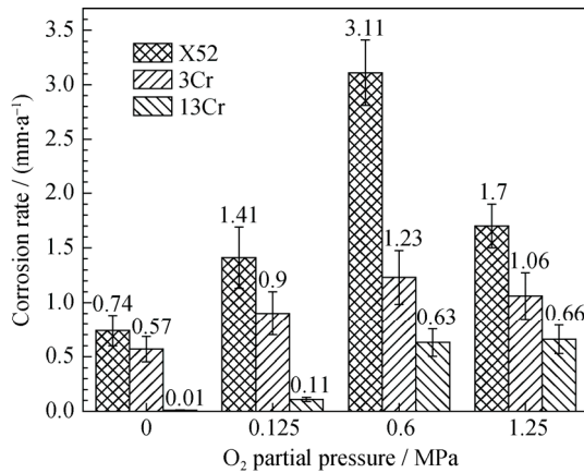
Fig. 12. Corrosion rates of X52, 3Cr, and 13Cr in different O 2 partial pressure environments; the error bar represents the maximum and minimum values.
