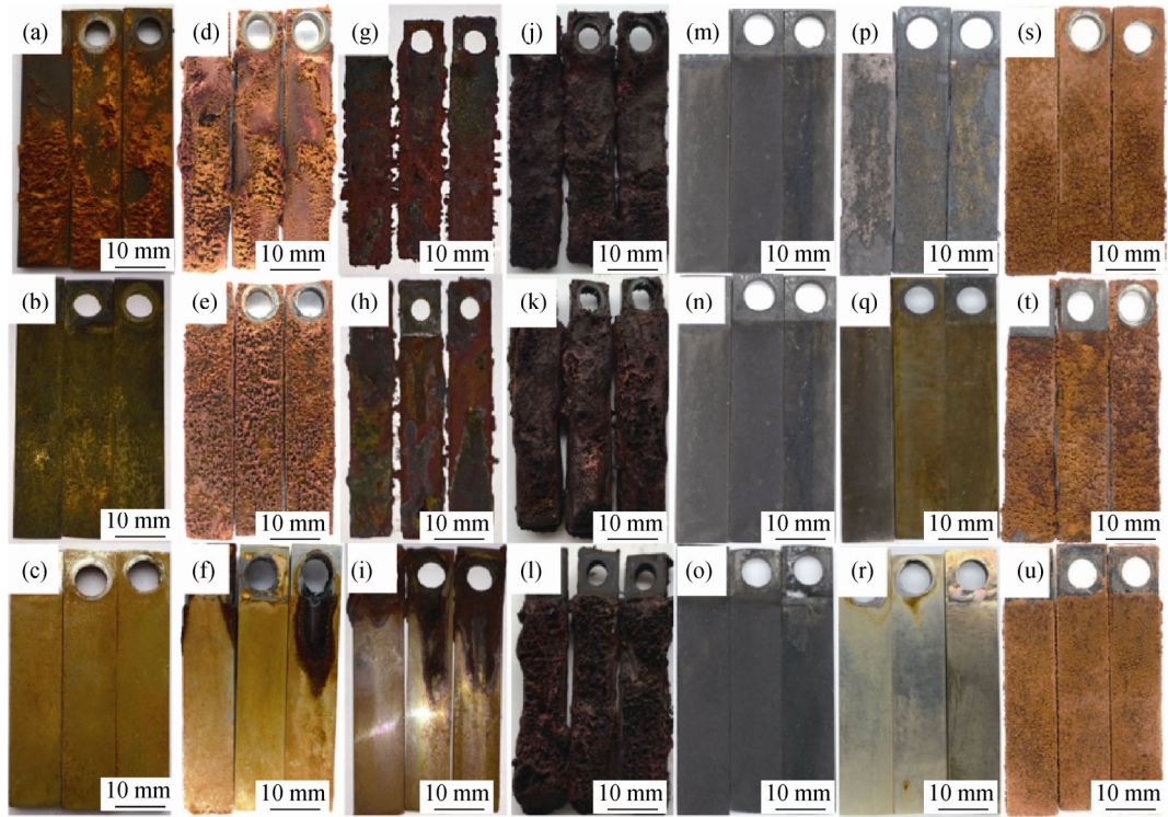
Fig. 2. Corrosion morphologies of different materials tested under different conditions shown in Table 2: (a–c) No. 1; (d–f) No. 2; (g–i) No. 3; (j–l) No. 4; (m–o) No. 5; (p–r) No. 6; (s–u) No. 7. The first, second, and third lines represent X52, 3Cr, and 13Cr, respectively.
