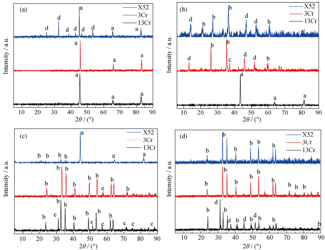
Fig. 5. XRD patterns of corrosion products formed at different test temperatures: (a) 25°C; (b) 60°C; (c) 100°C; (d) 140°C. The products are a—Fe, b—Fe 2 O 3 , c—Fe 3 O 4 , d—FeCO 3 , e—Cr 2 O 3 , and f—FeO(OH).
