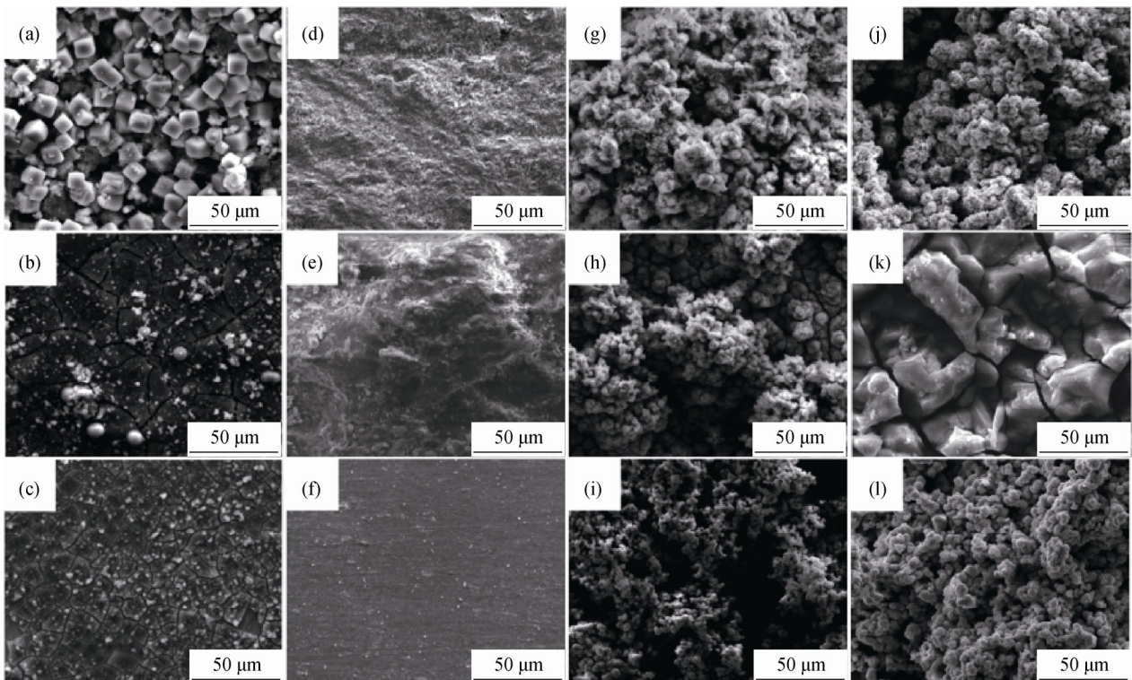
Fig. 3. Surface morphologies of the corrosion products of the tested materials: (a–c) No. 1; (d–f) No. 2; (g–i) No. 3; (j–l) No. 4. The first, second, and third lines represent X52, 3Cr, and 13Cr, respectively.
