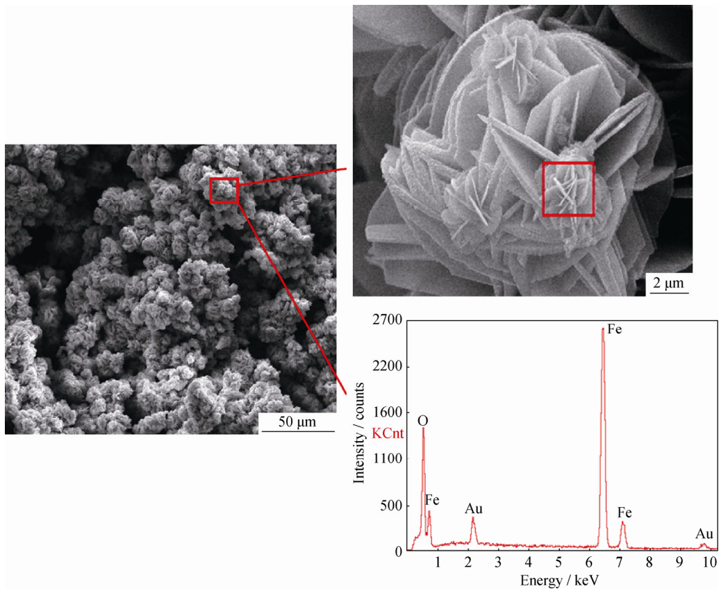
Fig. 4. EDS analysis of the flower-shaped corrosion product formed on the 3Cr specimen tested in No. 3 condition.
