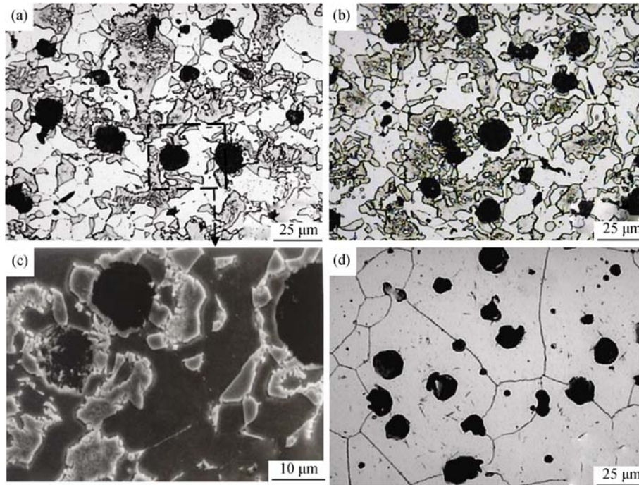
Fig. 5. Microstructures of the examined iron after annealing for 60 min at 920°C (a) and (c), 950°C (b), and 980°C (d).
