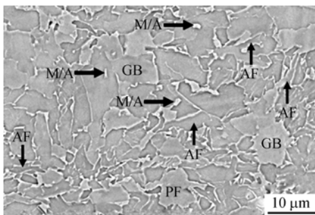
Fig. 4. SEM micrograph at the 1/4 thickness of the steel plate.
