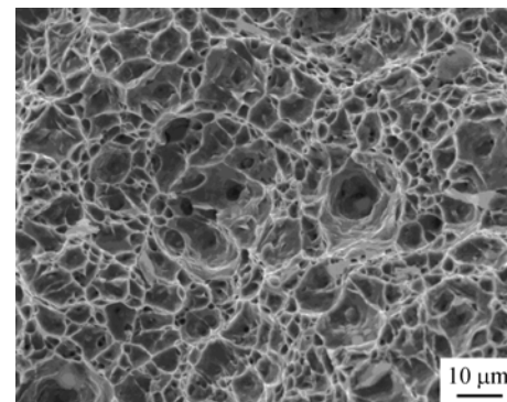
Fig. 10. SEM image of the tensile fracture specimen.
