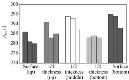
Fig. 8. Measured V-notch impact values at -40^{\circ}\text{C} along the plate thickness.
