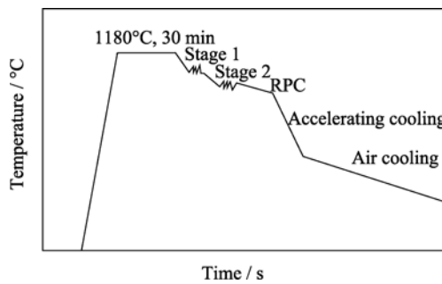
Fig. 1. Schematic illustration of an advanced TMCP-RPC process.
