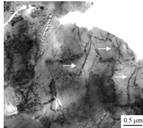
Fig. 7. Dislocation cells in the specimen.
