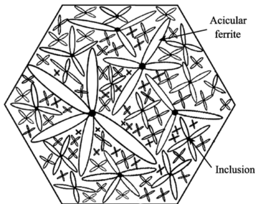
Fig. 9. Schematic illustration of the formation mechanism of interlocked acicular ferrite microstructures.
