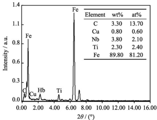
Fig. 6. EDXS results of Nb-Ti carbides.
