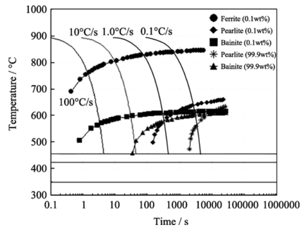
Fig. 2. Calculated CCT curves of the heavy plate steel.
