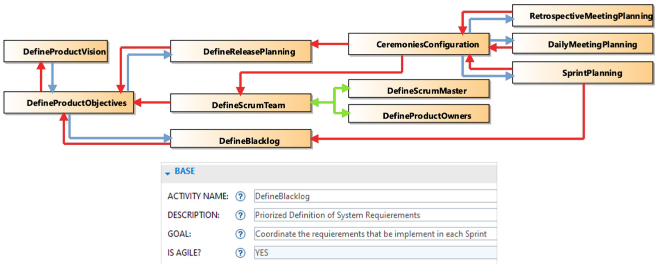
Fig. 8 Example model related to the pre-game phase of the Scrum method
