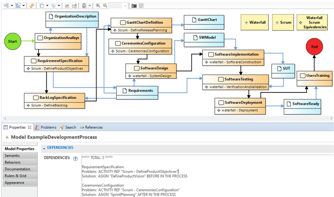
Fig. 11 Dependencies evaluation for the example process
