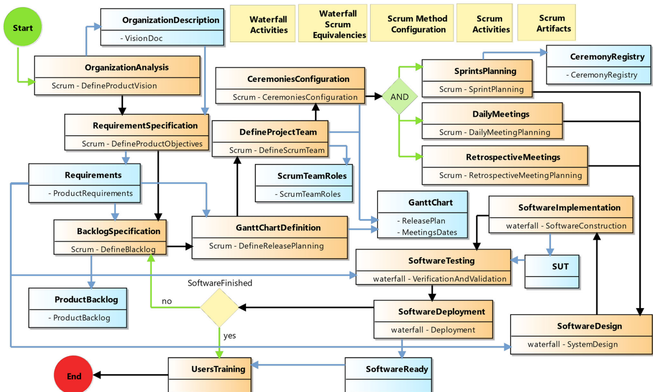
Fig. 15 Process obtained after the Analysis of method configurations
