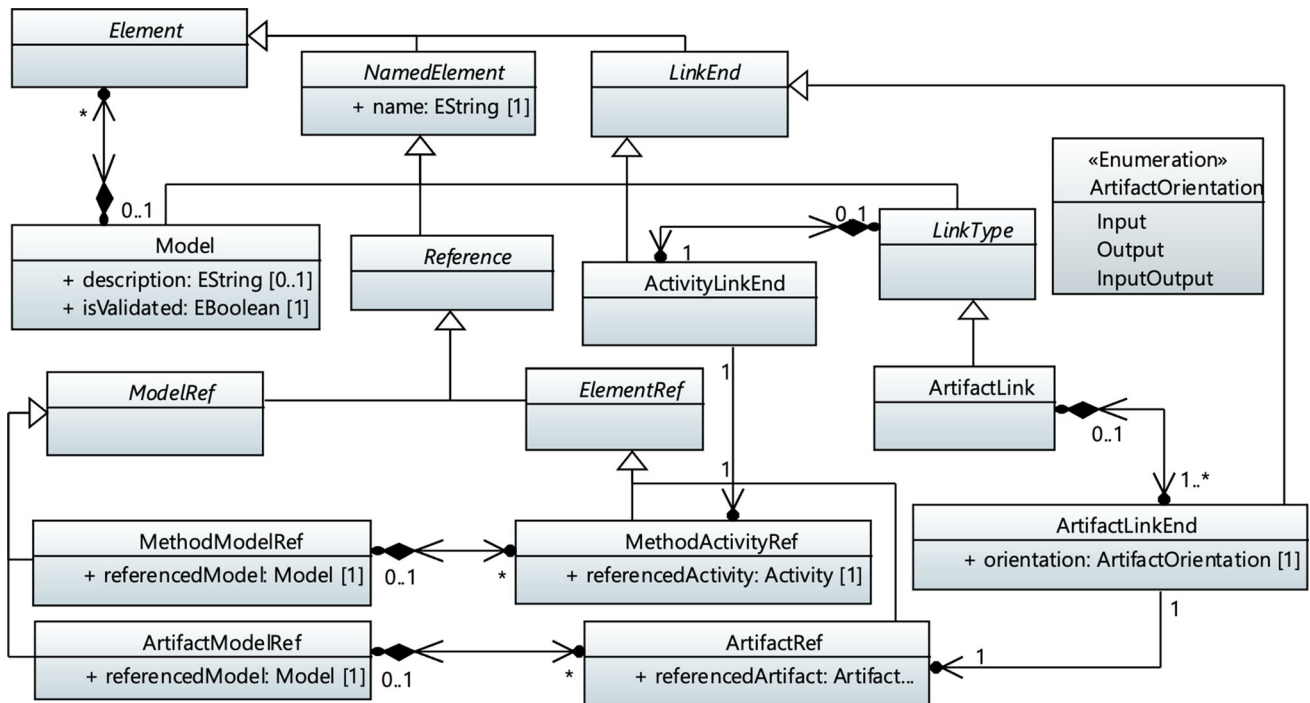
Fig. 5 Method configuration weaving metamodel
