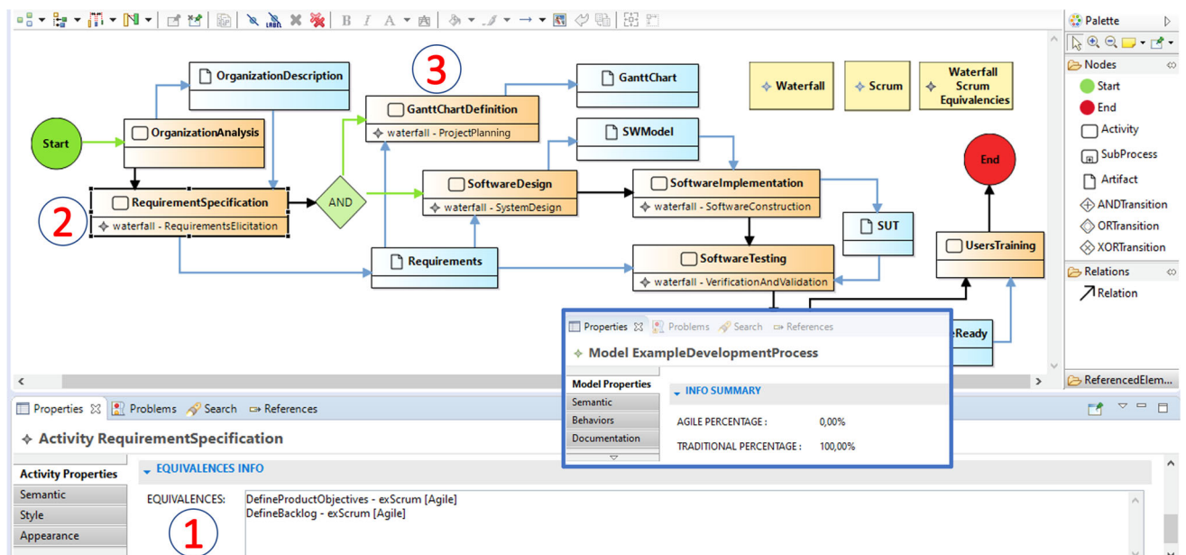
Fig. 10 Equivalency identification for the example process
