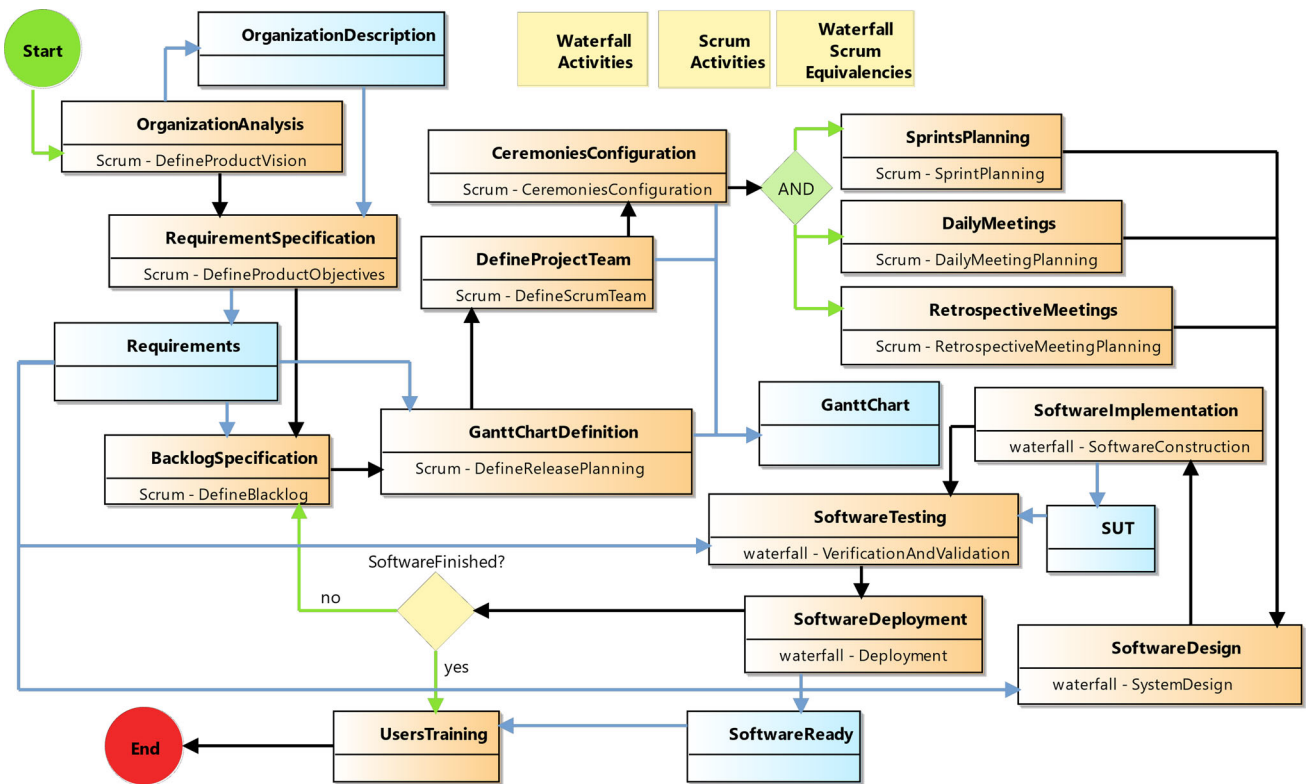
Fig. 12 Development process obtained after solving dependency issues
