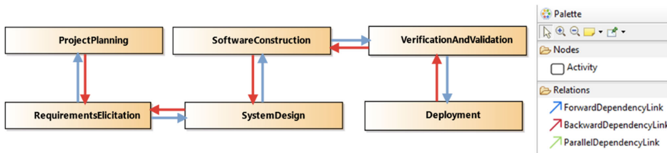
Fig. 7 Example of method definition for the Waterfall method
