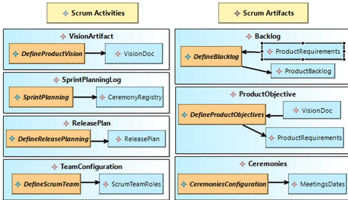
Fig. 13 Scrum method configuration model
