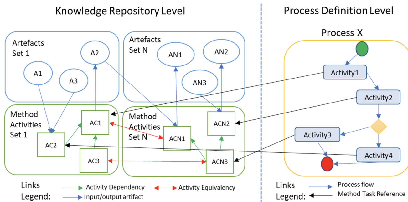
Fig. 2 Overview of SIAM conceptual architecture relationships
