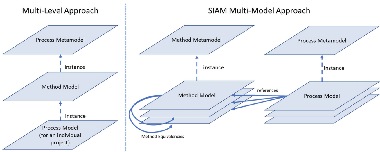
Fig. 1 Multi-level approach vs SIAM Multi-model approach
