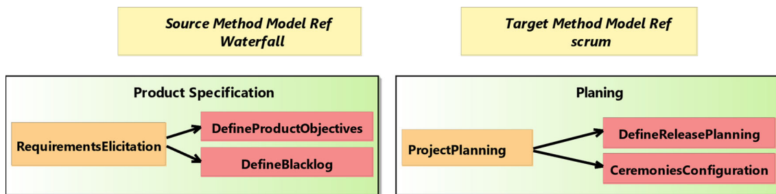
Fig. 9 Activities equivalency model defined between the Waterfall and Scrum methods
