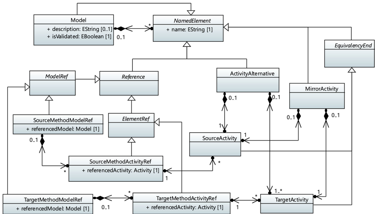
Fig. 4 Activity equivalency weaving metamodel
