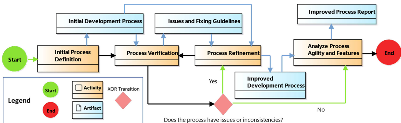
Fig. 6 SIAM Process configuration
