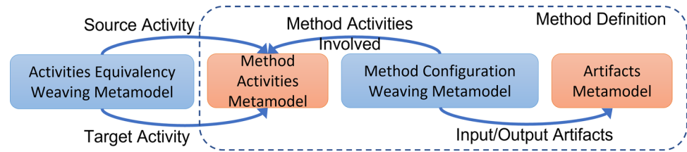
Fig. 3 Relationships between the metamodels of SIAM knowledge repository level
