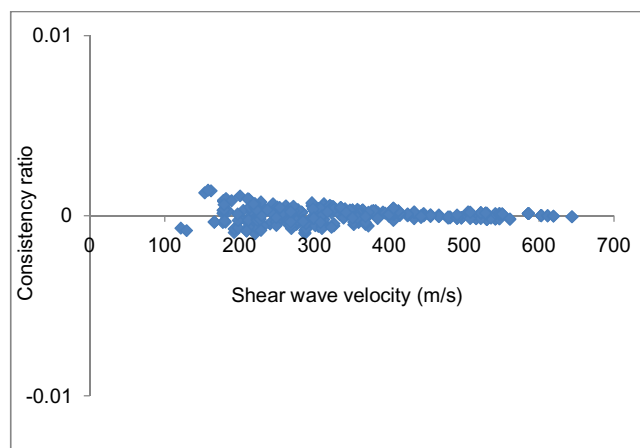
Fig.13. Typical plot of normalized consistency ratio of void ratio and V_s for all soil types
