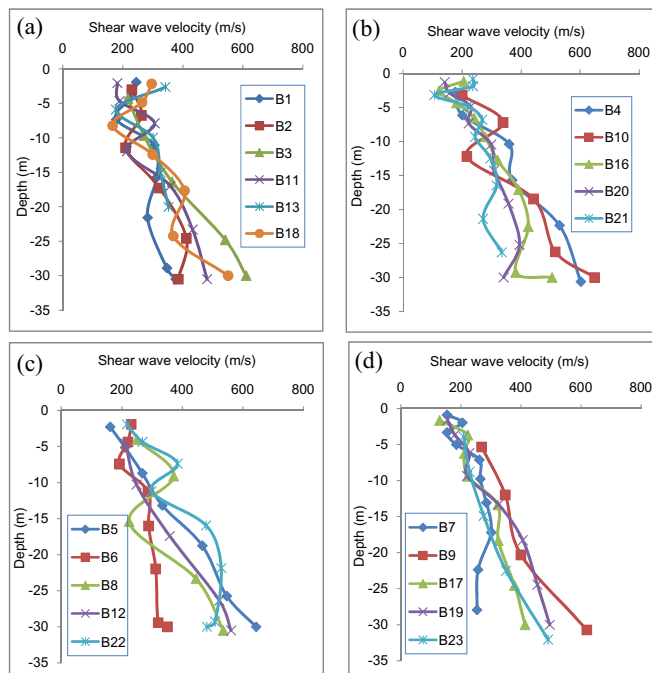
Fig.2a-d. Plot of shear wave velocity versus depth of data considered in the study
