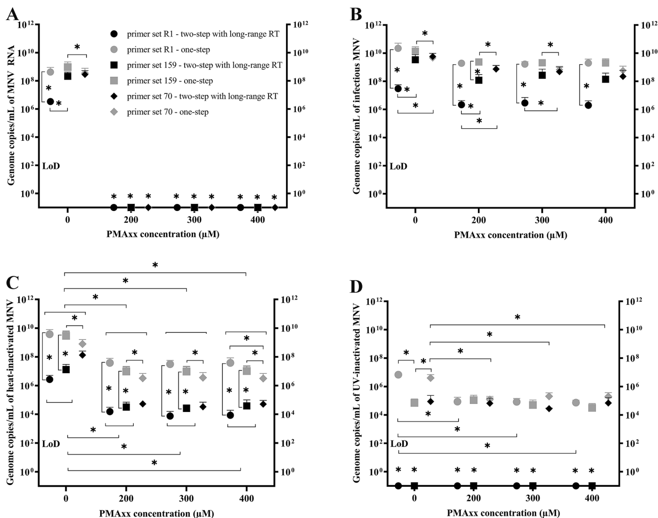
Fig. 2 Comparison between different concentrations (200, 300 and 400 µM) of PMAxx treatment on MNV in PBS and subsequent genome copy number quantification (gc/mL) with two processes: RT-qPCR with long-range RT and one-step RT-qPCR with three different pairs of primers; MNV RNA as positive control a , infectious MNV b , heat-inactivated MNV c and UV-inactivated d . The symbols represent the log genome copies of samples with standard deviation bars:
