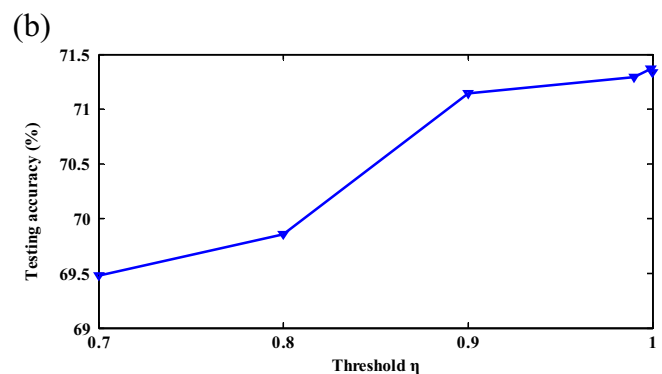
Fig. 6 Effect of the threshold \eta on the testing accuracy and number of selected hidden neurons. a Threshold \eta versus number of reserved hidden neurons. b Threshold \eta versus testing accuracy
