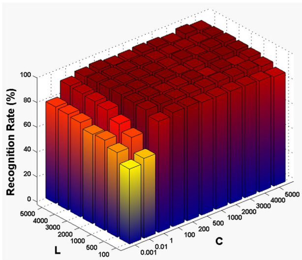
(a) ORL database
