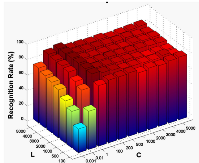
Fig. 5 The influence of tunable parameter ( L, C ) for DELM on different face database. a The ORL database, b the Extended Yale B database, c the CMU PIE database, and d the AR database
