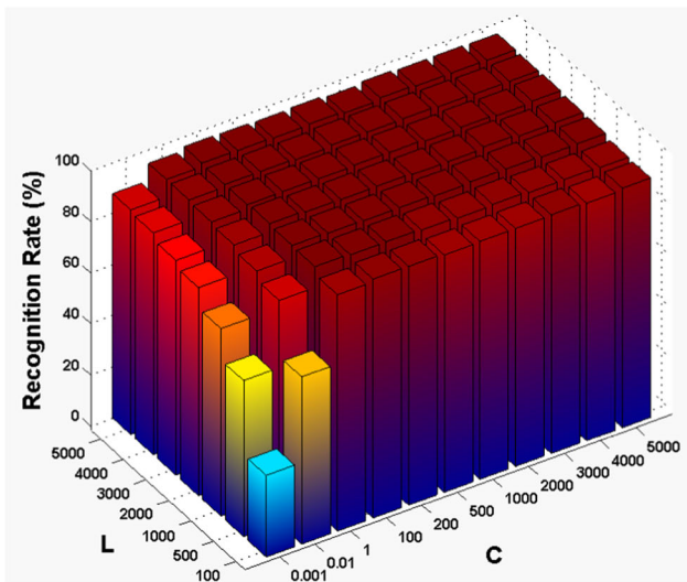
Fig. 5 The influence of tunable parameter ( L, C ) for DELM on different face database. a The ORL database, b the Extended Yale B database, c the CMU PIE database, and d the AR database
