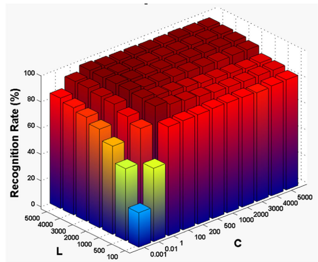
(b) Extended Yale B database
