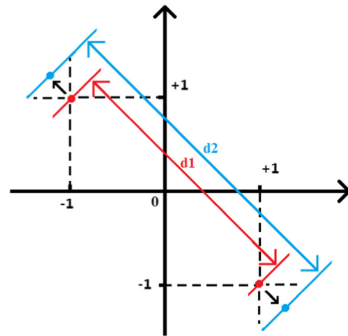
Fig. 1 A simplified illustration for proposed DELM. The regression labels in classic ELM are denoted as red points . After dragged to the blue ones , the distance between the samples' regression labels is enlarged. With this strategy, DELM is expected to fully exploit the discriminative information in data
