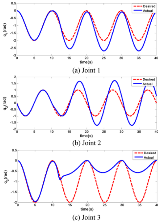
Fig. 7 Joint angle trajectories when fault \phi_2 occurs
