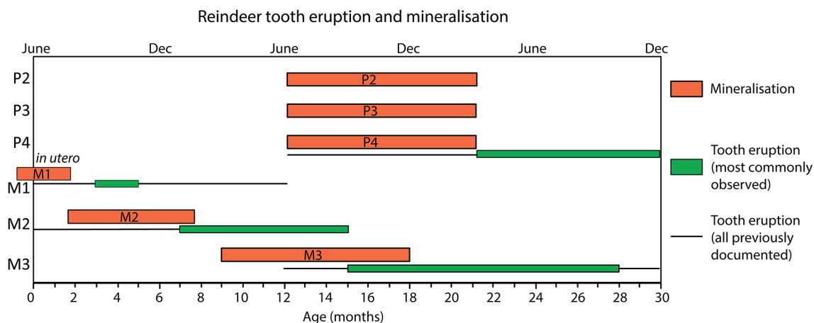
Fig. 2 Reindeer tooth mineralisation and eruption intervals. Mineralisation intervals based on estimates from cervids, previous isotopic studies of reindeer and, for P2 and P3, the intra-tooth seasonality data
