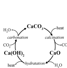
Lime production
