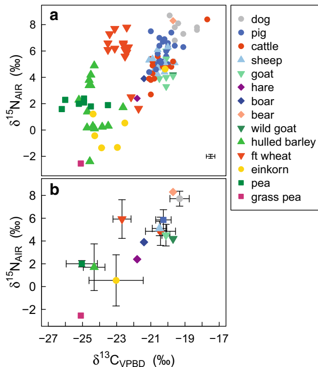
Fig. 3 All plant and animal \delta^{13}\text{C} and \delta^{15}\text{N} values from Neolithic Kouphovouno. Samples KFO34 and KFO50 are not included, because they only yielded a reliable \delta^{15}\text{N} value. a Individual measurements, b means and standard deviations of each species. The dataset includes samples measured previously (28 plants and 68 animals, Vaiglova et al. 2014a); the previous plant measurements were corrected here using the more recent charring correction (see “Materials and methods”). Measurement error is shown in the bottom-right of a
