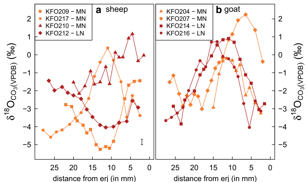
Fig. 9 Sequential tooth enamel carbonate \delta^{18}\text{O} measurements of sheep (a) and goats (b) from Middle (MN) and Late Neolithic (LN) levels at Kouphovouno. Measurement error is shown in the bottom-right of a
