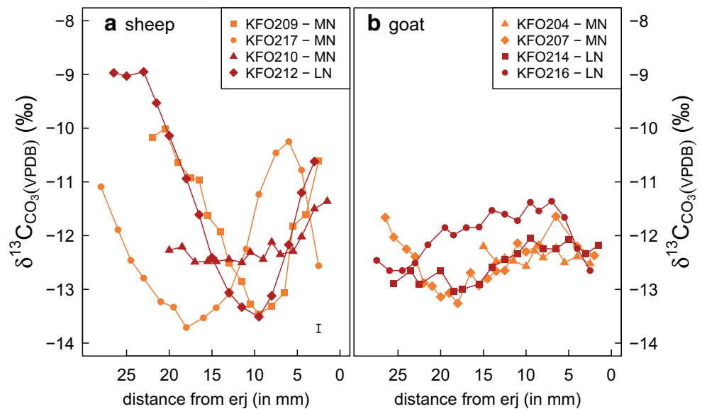
Fig. 8 Sequential tooth enamel carbonate \delta^{13}\text{C} values of sheep (a) and goats (b) from Middle (MN) and Late Neolithic (LN) levels at Kouphovouno. Measurement error is shown in the bottom-right of a
