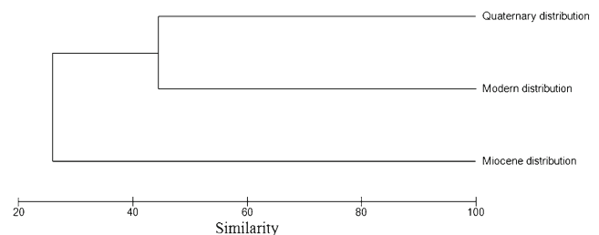
Fig. 7 Cluster analyses of genera composition of Quaternary, modern and Miocene based on presence–absence data and Bray–Curtis similarities
