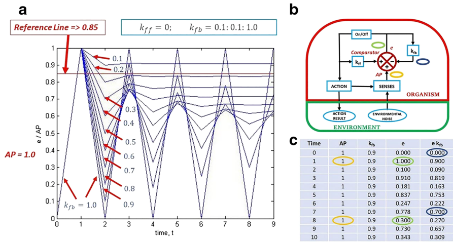
Fig. 3 a The effect of changing k_{fb} in the generation of richer dynamical behaviours. b Color-coded one-parameter feedback loop. c Color-coded variation of one-parameter feedback loop for k_{fb} = 0.9
