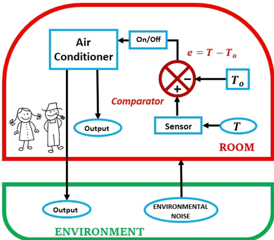
Fig. 1 A one-parameter feedback loop simulation of a homeostatic control mechanism (thermostat) associated with a room air conditioning system
