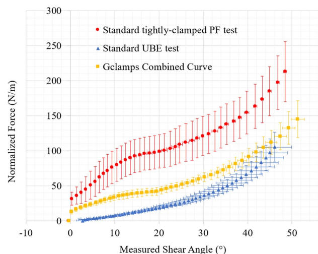
Fig. 16 Comparison of normalized force vs measured shear angle curves of standard tightly-clamped PF test, standard UBE test and resultant G-clamped PF test combined curve
