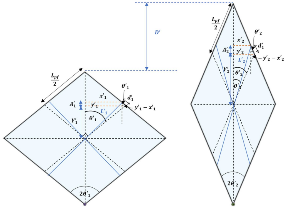
Fig. 18 Negative pre-displaced of the PF rig (a) Loaded specimen to the negative pre-displaced rig (b) The picture frame rig after crosshead displacement, D
