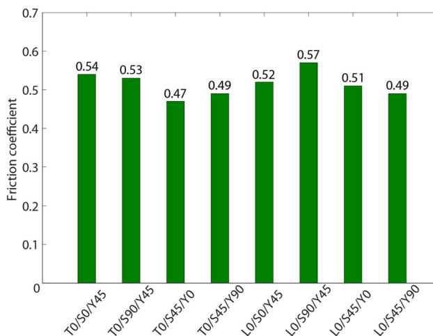
(b) Average friction coefficients in different orientations
