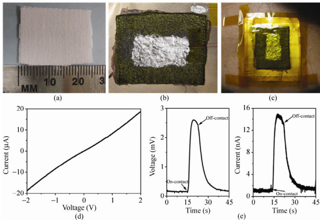
Figure 4 (a) Photograph of a fixed-area fabric. (b) Photograph of the device fabricated onto a flexible Kapton substrate. (c) Photograph of the device attached on the human body. (d) I - V characteristics of the device. (e) Electrical output voltage and current when a cooler was contacted with the outer surface of the device
