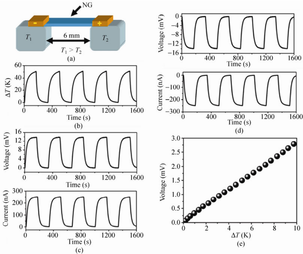
Figure 2 (a) Schematic diagram of the measurements. (b) The cyclic change in temperature difference across the device. The output voltage and current of the TENG in forward connection (c) and reversed connection (d) to the measurement system. (e) The output voltage of the TENG as a function of change in temperature difference across the device
