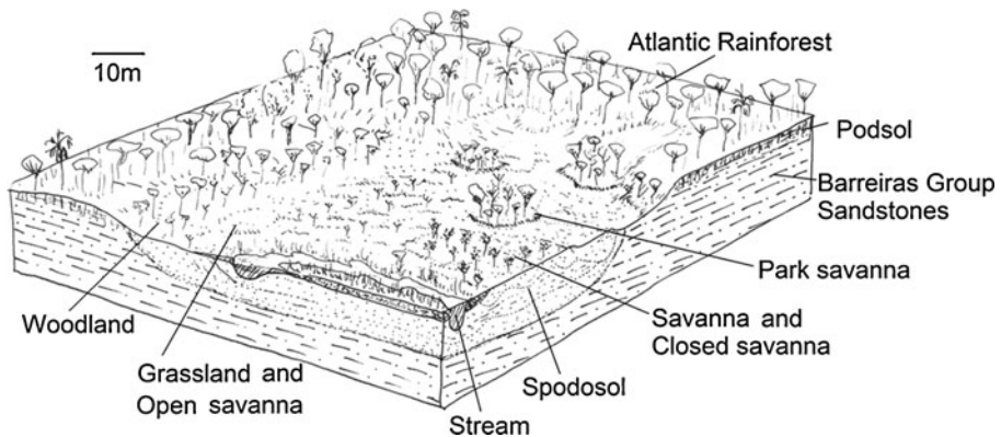
Fig. 1 Diagram of a Mussununga with surrounding Atlantic Rainforest. Soil names are according to the U.S. system of soil classification
