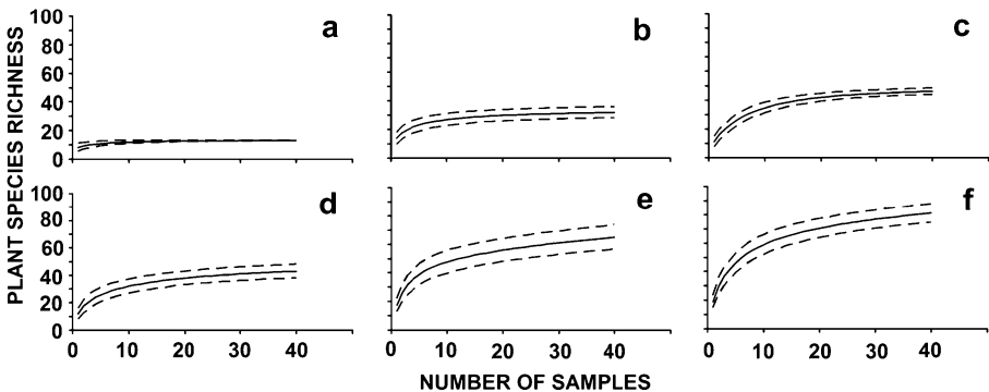
Fig. 4 Estimates of richness using the Mao Tau estimator by means of simulations for 40 plots in each of the six vegetation forms of Mussununga: a grassland, b open savanna, c savanna, d closed savanna, e park savanna, f woodland. Solid lines are mean values of richness; dashed lines are confidence intervals of 95% ( \pm 1.96 s.d.)
