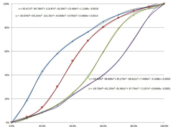
Fig. 7. Regression Equations for Huff Distributions in the City of Jeongjeup
