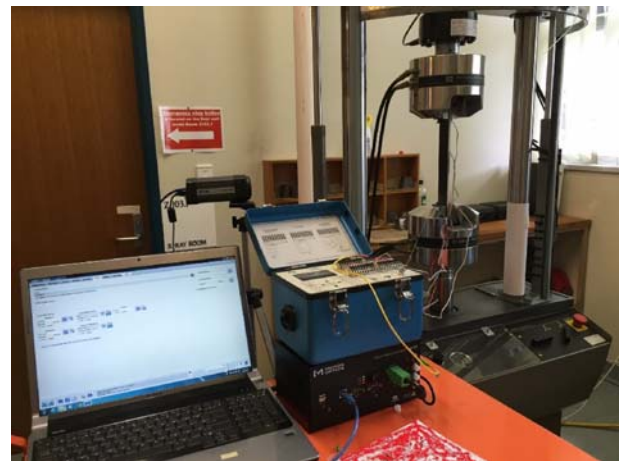
Fig. 5 Experimental setup
