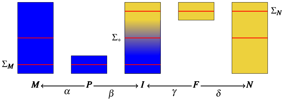
Fig. 4 The chain of Cauchy morphisms in the proof of Theorem 4.4
