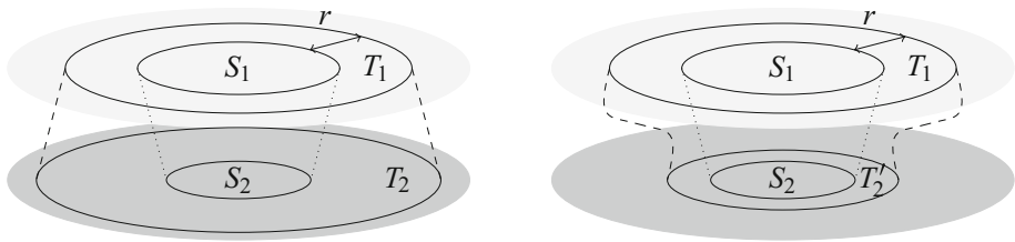
Fig. 5 Illustration of the ‘inflationary’ proof of the distal split bound
