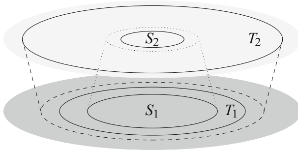
Fig. 2 Regular Cauchy pairs with (S_1, T_1) \prec_M (S_2, T_2)
