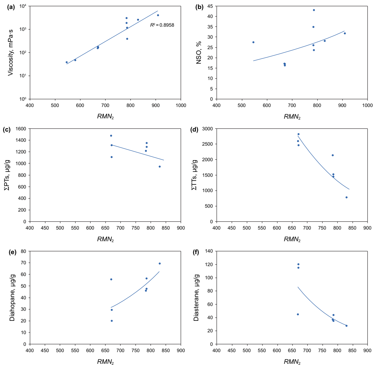
Fig. 10 Correlations of the refined Manco number (MN 2 ) with oil viscosity (a), NSO content (b), summed pentacyclic terpane (c) and tricyclic terpane concentrations (d), and absolute concentrations of diahopane (e) and diasteranes (f). All the concentration data were cited after (Chang et al. 2018)
