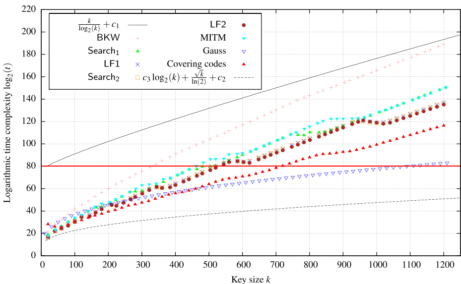
Fig. 1 Time Complexity of LPN Algorithms on instances LPN_{k, \frac{1}{\sqrt{k}}}
