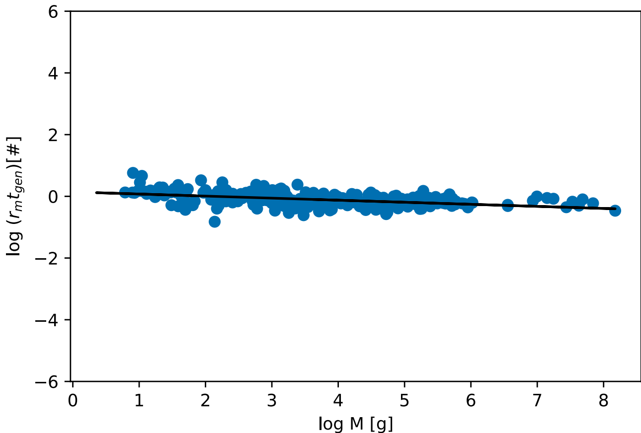
Fig. 3 Generation times ( t_{gen} ) times the maximum population growth rates ( r_m ) for mammals, compiled by Duncan et al. (2007). The solid line denotes r_m t_{gen} = 1.38 M^{-0.067} , which is the best fit to the data and has an
