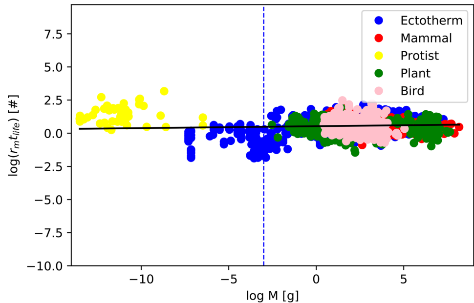
Fig. 2 Lifetime growth: intrinsic (maximum) population growth rates ( r_m ) multiplied by the corresponding lifespans ( t_{life} ) for all types of living organisms, ranging from protists to mammals and birds, compiled by Hatton et al. (2019). The solid black line corresponds to the best fit to the data, with no residual slope with body mass, r_m t_{life} = 3.35 M^{0.01} , as expected from Eq. 8, with a scatter of 0.5 dex. The dashed blue line denotes the mass scale of 10^{-3} grams, which corresponds to the scale associated with the smallest organisms with hearts, to which the present analysis is restricted
