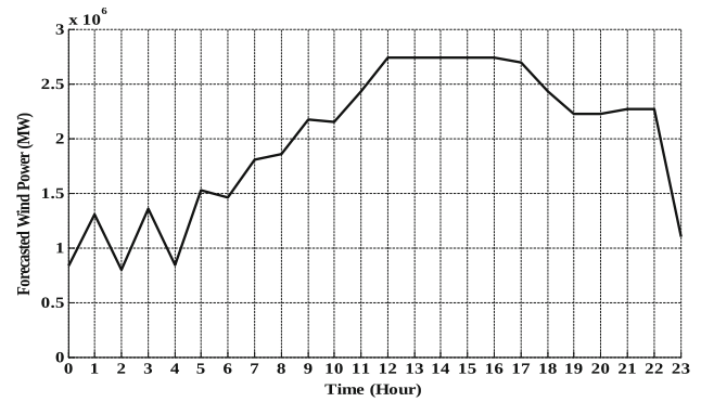
Figure 3. Projected wind power for a typical day.
