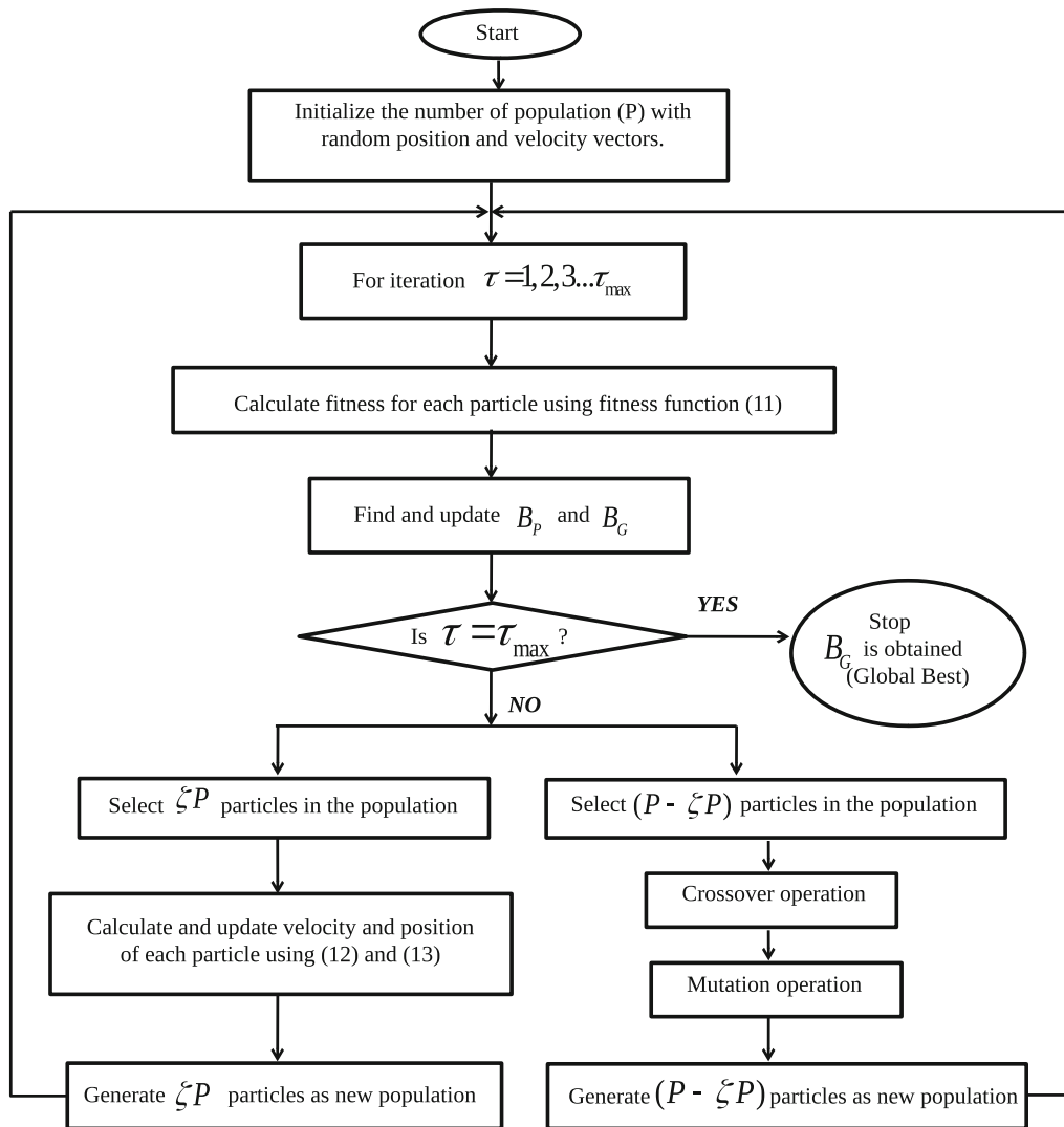
Figure 2. Flowchart of hybrid GA-PSO algorithm.
