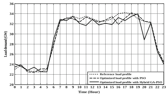
Figure 5. Optimized load demand pattern of a typical day with PSO and hybrid GA-PSO.
