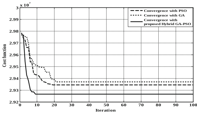
Figure 6. Cost convergence characteristics with different optimization algorithms.
