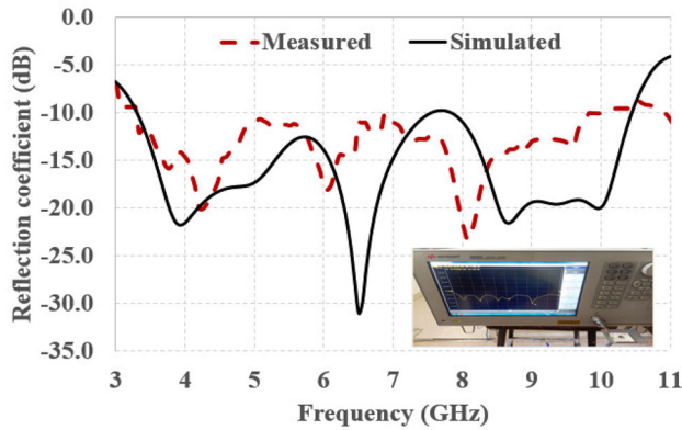
Figure 7. Simulated and measured S-parameter of the proposed hollow DRA.
