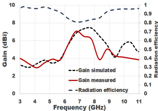
Figure 8. Measured and simulated gain, and simulated radiation efficiency.
