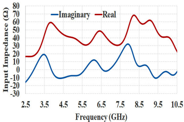
Figure 5. Simulated Antenna impedance plot.
