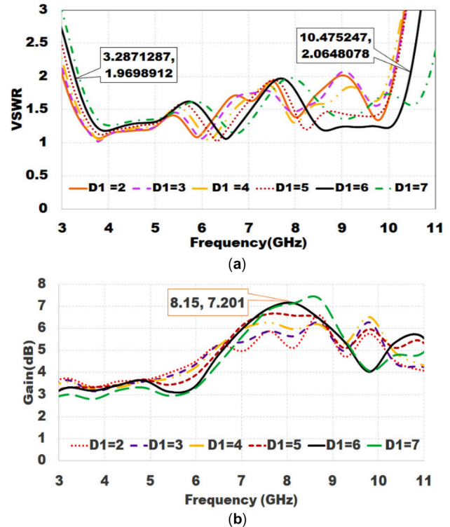
Figure 2. Effect of Hollow DR antenna A. VSWR, B. Gain.
