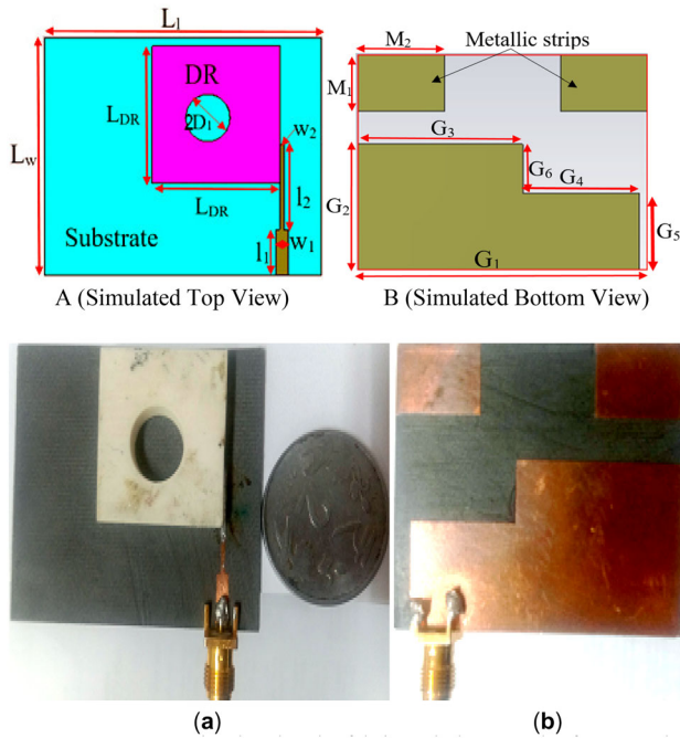
Figure 1. Antenna simulated and a fabricated photograph of proposed hollow antenna. A. Top view and B. back view.
