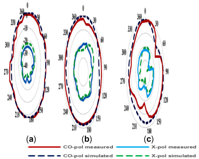
Figure 9. Simulated and measured co and X polarization pattern of antenna A. 4.1 GHz, B. 6.2 GHz, C. 8.1 GHz.
