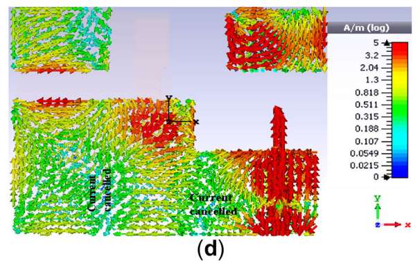
Figure 4. Surface current distribution at A 3.8 GHz, B 6.4 GHz, C 8.8 GHz, D 10 GHz.
