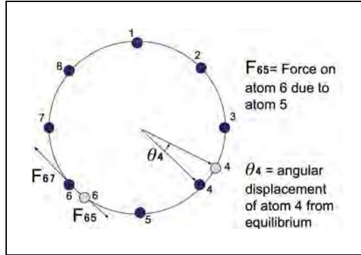
Figure 1. Toda chain of N = 8 particles with periodic boundary conditions.
