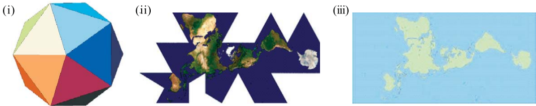
Figure B. (i) An icosahedron with 20 faces, (ii) the surface of the Earth projected onto an icosahedron and developed in a particular way, (iii) Dymaxion projection of the Earth where the entire world looks like an island in a great ocean.
