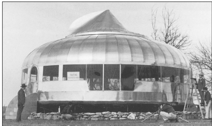
Figure 8. Wichita House, one of two prototypes built of the Dymaxion house.
