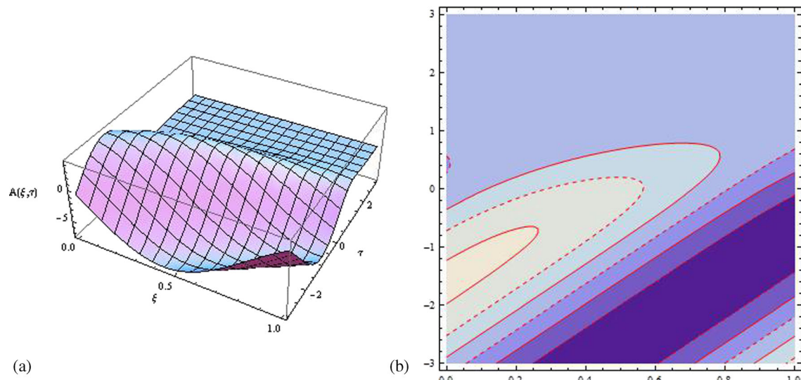
Figure 5. The velocity potential (50) with different shapes are plotted: (a) travelling wave solutions, (b) contour plot.
