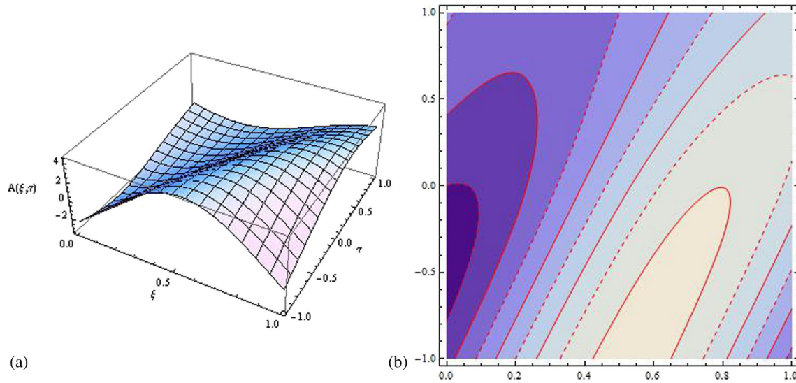
Figure 4. The velocity potential (49) with different shapes are plotted: (a) travelling wave solutions, (b) contour plot.
