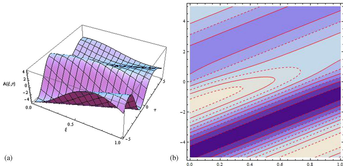
Figure 3. The velocity potential (43) with different shapes are plotted: (a) periodic travelling wave solutions, (b) contour plot.
