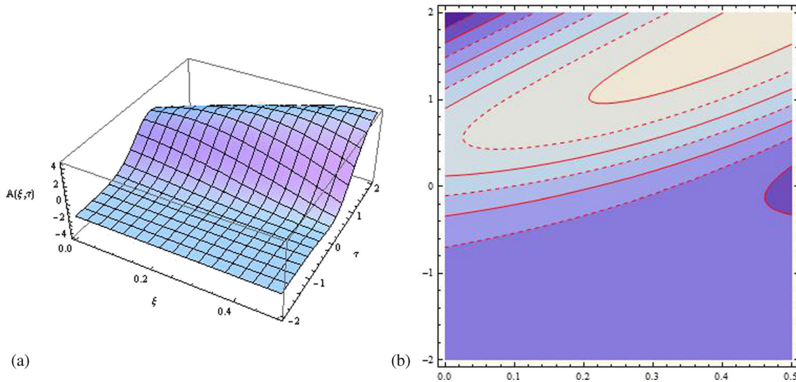
Figure 6. The velocity potential (51) with different shapes are plotted: (a) travelling wave solutions, (b) contour plot.
