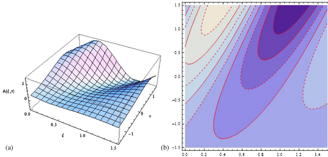
Figure 7. The velocity potential (55) with different shapes are plotted: (a) travelling wave solutions, (b) contour plot.
