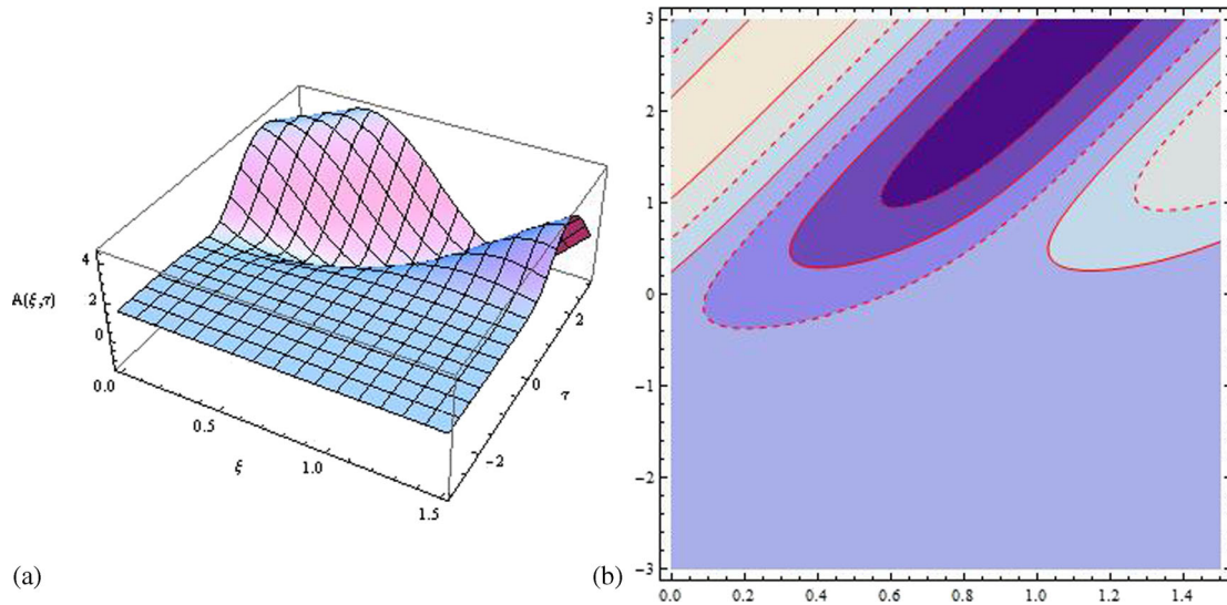
Figure 2. The velocity potential (43) with different shapes are plotted: (a) solitary wave solutions, (b) contour plot.
