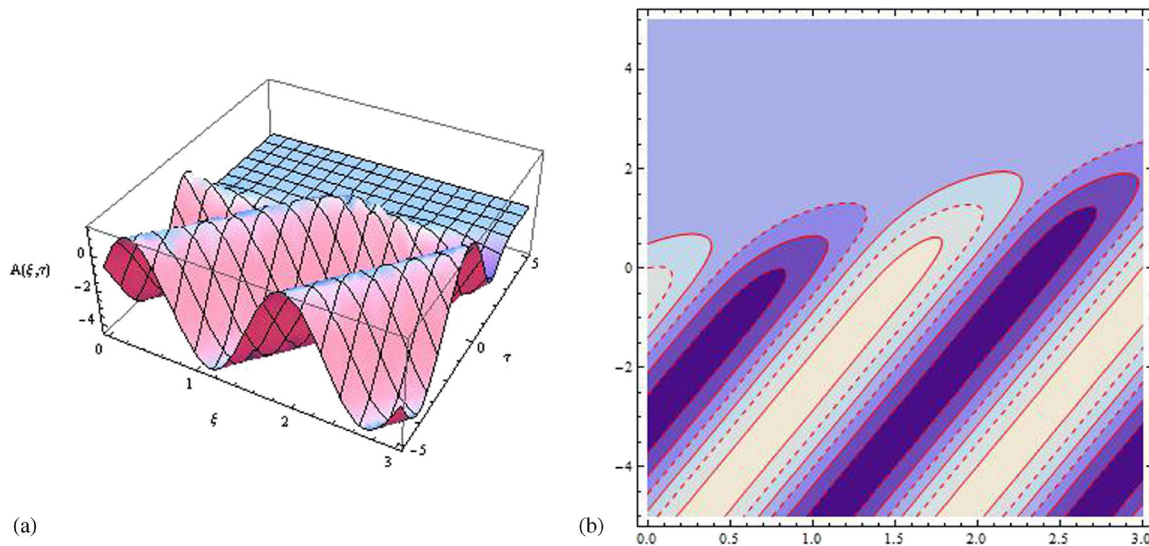
Figure 1. The velocity potential (42) with different shapes are plotted: (a) solitary wave solutions, (b) contour plot.
