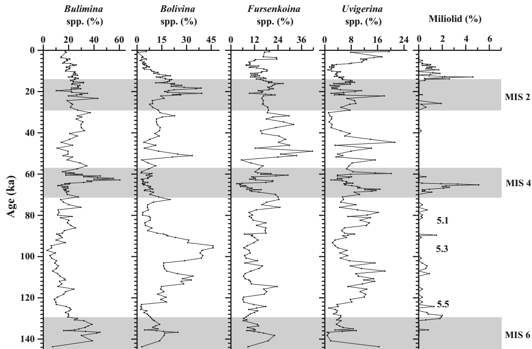
Figure 3. Temporal variation in relative abundances of major benthic foraminiferal genera at ODP Hole 723A (even numbered grey horizontal bars represent glacial stages).
