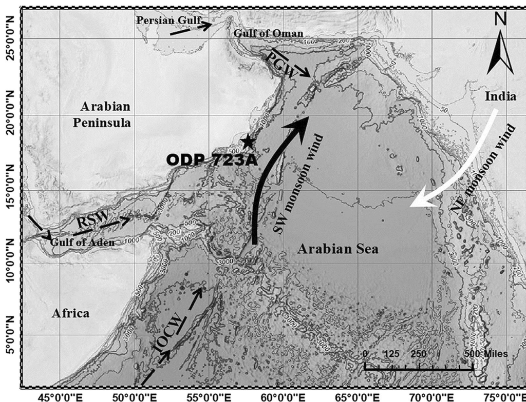
Figure 1. Location map of ODP Hole 723A in the northwestern Arabian Sea. Black arrow represents southwest monsoon and white arrow indicates northeast monsoon.
