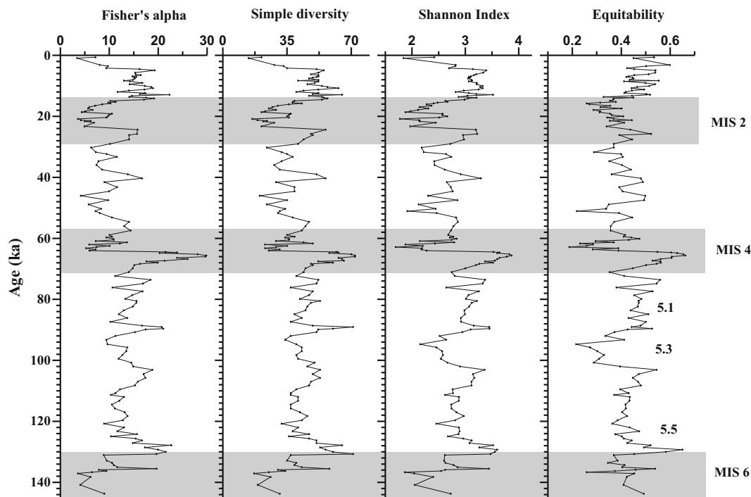
Figure 4. Temporal variation in the values of different diversity indices (Fisher's alpha index ( \alpha ); Simple diversity ( S ); Shannon index ( H ) and equitability ( E ) (even numbered grey horizontal bars represent glacial stages).
