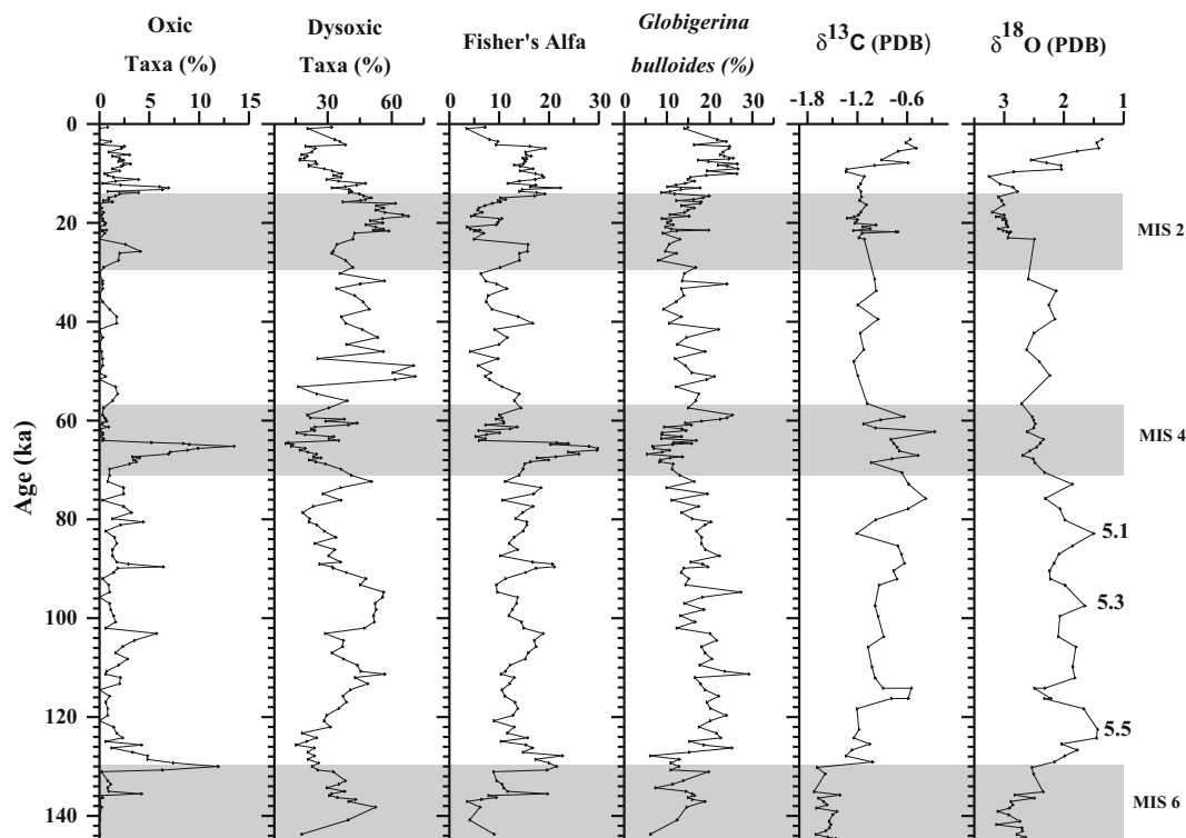
Figure 5. Temporal variation in relative abundances of Oxidic taxa (%), Dysoxic taxa (%), Fisher's alpha ( \alpha ), Globigerina bulloides (%); benthic \delta^{13}\text{C} and \delta^{18}\text{O} at ODP Hole 723A (Niitsuma et al. 1991) (even numbered grey horizontal bars represent glacial stages).
