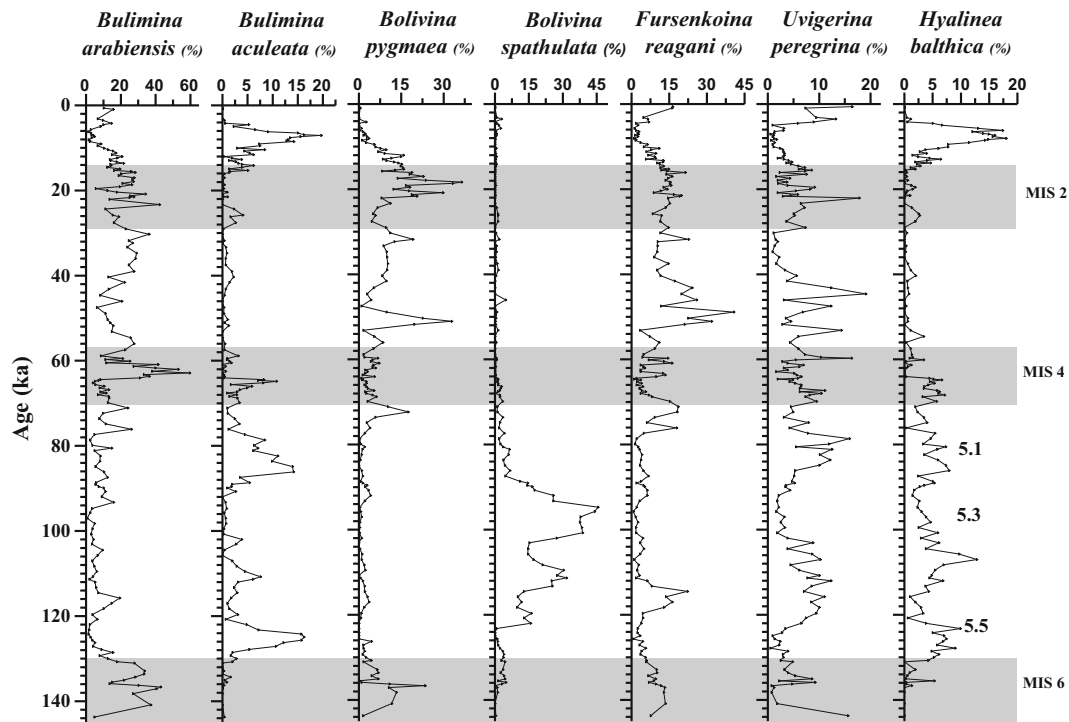
Figure 2. Temporal variation in relative abundances of major benthic foraminiferal species at ODP Hole 723A (even numbered grey horizontal bars represent glacial stages).
