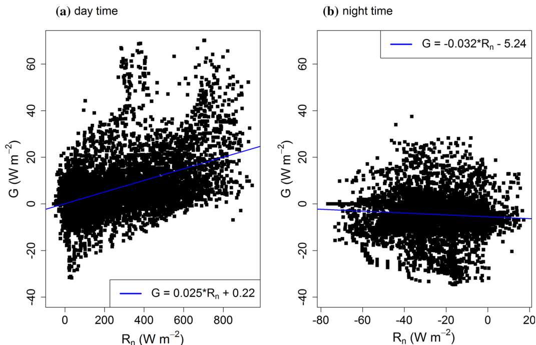
Figure 5. Scatter plots and linear fits between net radiation ( R_n ) and soil heat flux ( G ) during (a) daytime and (b) nighttime for KNP in 2016. Daytime is defined using ( R_{SW(in)} \geq 20 \text{ W m}^{-2} ). Governing equation for each of the fits is given in the respective figure legends.
