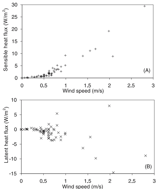
Figure 4. Variation of daily mean (A) sensible heat flux and (B) latent heat flux with wind speed at Dhundi (13 January–12 April 2005).
