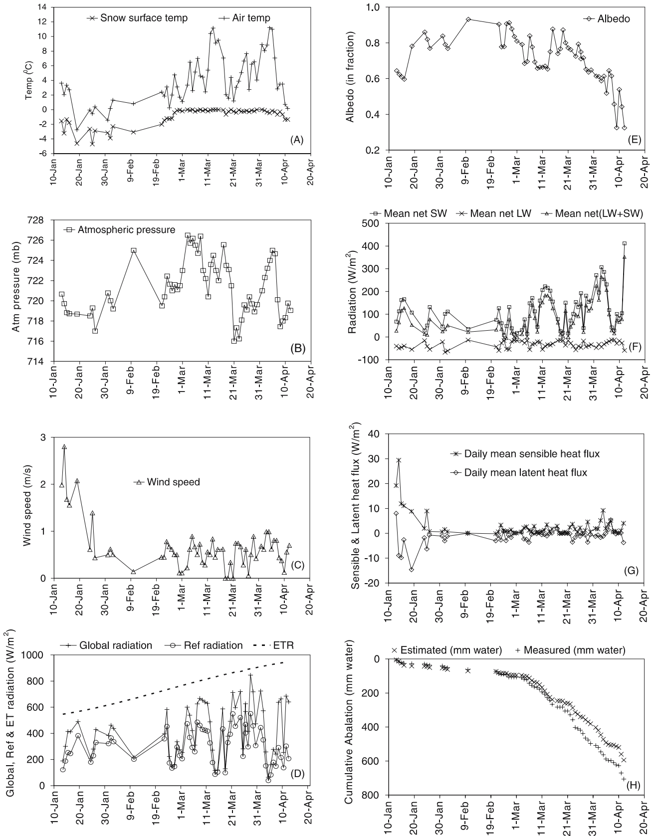
Figure 2. (A) Daily mean snow surface temperature and daily mean air temperature. (B) Daily mean atmospheric pressure. (C) Daily mean wind speed. (D) Daily mean global, reflected radiation and extra terrestrial radiation (ETR). (E) Daily mean albedo. (F) Daily mean net shortwave, net longwave and mean net radiation (net SW+ net LW) energy flux. (G) Daily mean sensible heat flux and latent heat flux. (H) Comparison of cumulative estimated snow-melt and cumulative ablation. (All parameters A-H at Dhundi for period 13 January to 12 April 2005.)
