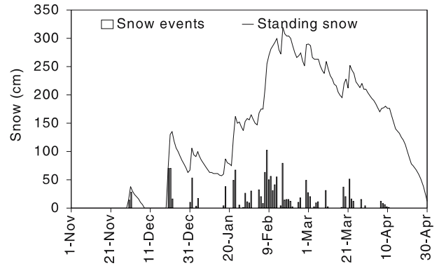
Figure 1. Standing snow and fresh snow events at Dhundi Observatory, winter 2004–2005.
