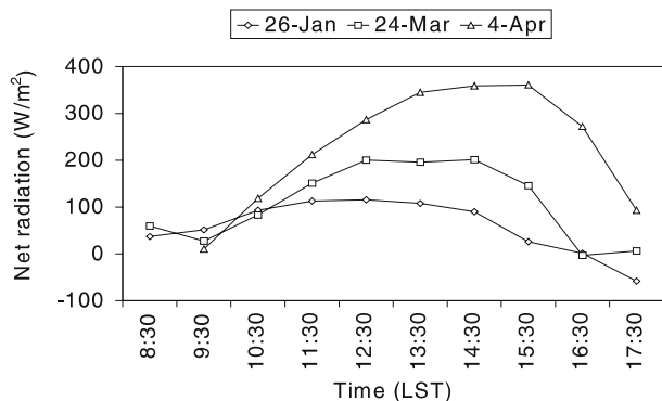
Figure 3. Variation of net radiation for three clear days of the season at Dhundi (13 January–12 April 2005).
