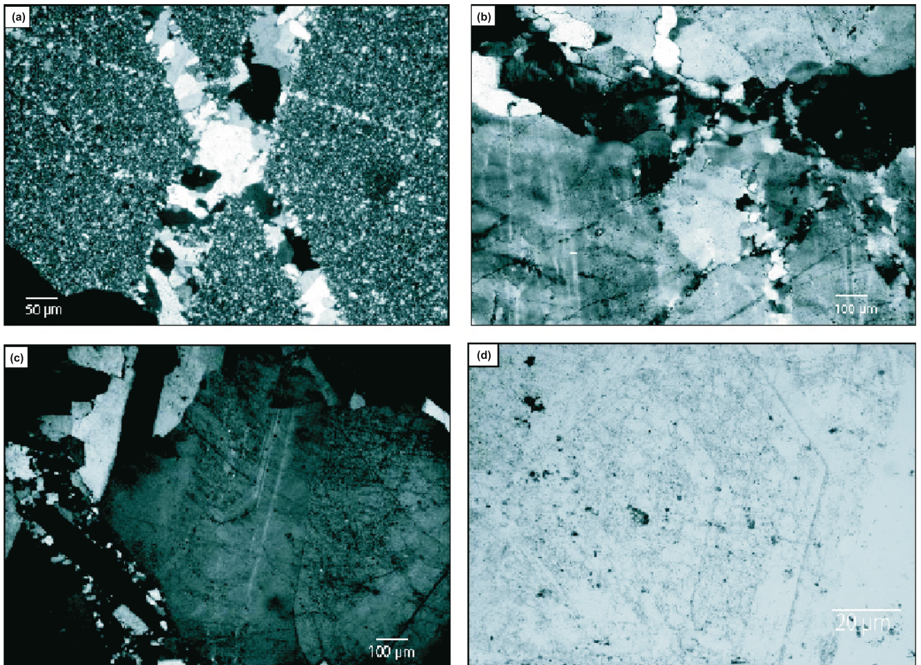
Figure 4. Photomicrographs under crossed nicols. (a) Thin cross-cutting veins of crystalline quartz within a sample of giant quartz vein of fine-grained ('cherty') variety. (b) Giant quartz vein sample showing undulose extinction and well-developed deformation lamellae suggesting crystal plastic deformation of quartz. (c) Zoned quartz grain (centre) with zones of variable thickness which is cut across by a late quartz vein (left). (d) Close-up photomicrograph of a zoned quartz grain. Zoning may be the result of trace element compositional changes across the grain profile and/or abundance of sub-micron sized inclusions.
