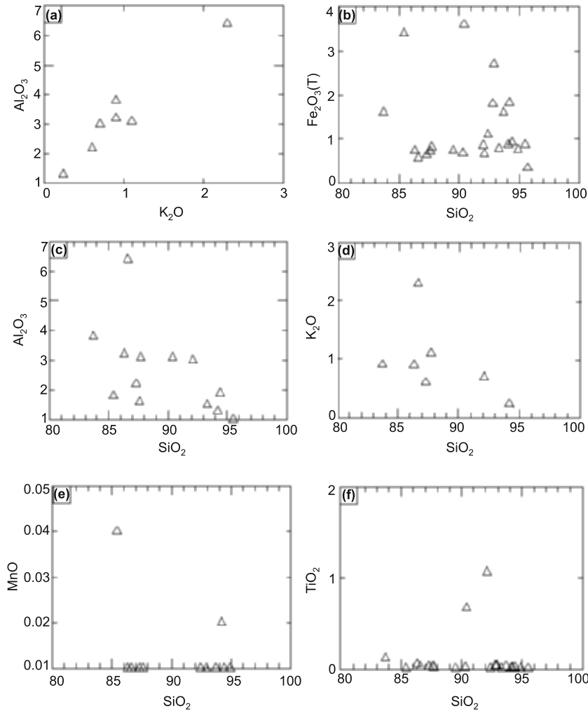
Figure 5. Bivariant major oxide plots (a–f) of GQVs. Only those samples with appreciable content of different oxides have been plotted. Positive correlation is seen between \text{Al}_2\text{O}_3 and \text{K}_2\text{O} (5a). \text{SiO}_2 versus major oxides (5b–5f) depict a scatter for elements such as \text{Fe}_2\text{O}_3 (T), \text{Al}_2\text{O}_3 , \text{K}_2\text{O} , \text{MnO} and \text{TiO}_2 , respectively.
