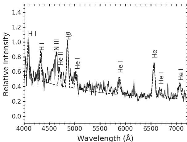
Figure 5. Best-fit modelled spectrum (dash line) plotted over the observed spectrum (continuous line) for day 1.52 (8.61 Nov 2018) of 2018 outburst of M31N 2008-12a.
