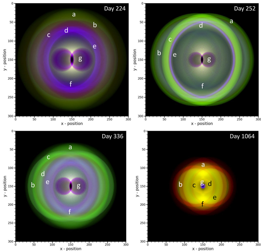
Figure 4. Evolution of the geometry of ejecta of T Pyx on day 224 ( top left ), 252 ( top right ), 336 ( bottom left ), and 1064 ( bottom right ) in the two-dimensional plane with X-axis being the line-of-sight direction and Y being the axis perpendicular to that of the plane of sky and line-of-sight. The lines corresponding to different colours are marked to show the spatial distribution of emission in the structure. There is formation of multiple equatorial rings and also the spatial distribution of the ionized lines as the system evolves. Here, a: [O III] \lambda 5007 , b: [O III] \lambda 4959 , c: H \alpha , d: H \beta , e: N III \lambda 4638 , f: [N II] \lambda 5755 , g: He II \lambda 4686 . Only dominant lines are marked. Here, 1 unit of x and y position correspond to x_{224} = 6.3 \times 10^{12} cm, x_{252} = 1.41 \times 10^{13} cm, x_{336} = 2.09 \times 10^{13} cm, and x_{1064} = 1.66 \times 10^{12} cm.
