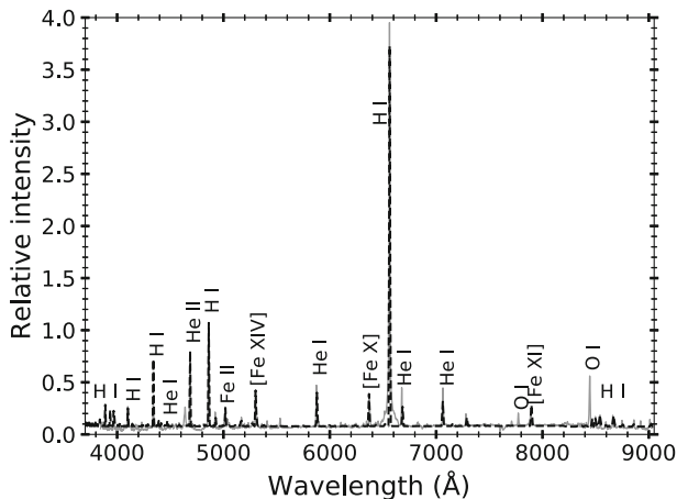
Figure 2. Best-fit modelled spectrum (dash line) plotted over the observed spectrum (continuous lines) for day 19 (16 September 2019) of 2019 outburst of V3890 Sgr.
