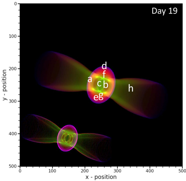
Figure 3. Morphology of the ejecta of V3890 Sgr on day 19 during its 2019 outburst obtained using the optical spectrum in the two-dimensional plane with X-axis being the line-of-sight direction and Y being the axis perpendicular to that of the plane of sky and line-of-sight. Here, 1 unit of x and y corresponds to 8.13 \times 10^{11} cm. The labels marked represent a: Fe II, b: He I, c: He II, d: [Fe VII], e: [Fe X], f: [Fe XI], g: [Fe XIV], h: H I, i: [N II].
