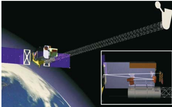
Figure 5. Spacecraft concept for advanced large-aperture coronagraphs. The inset is a diagram of the telescope/spectrometer unit of a next generation ultraviolet coronagraph spectrometer (from Kohl et al. 2006).
