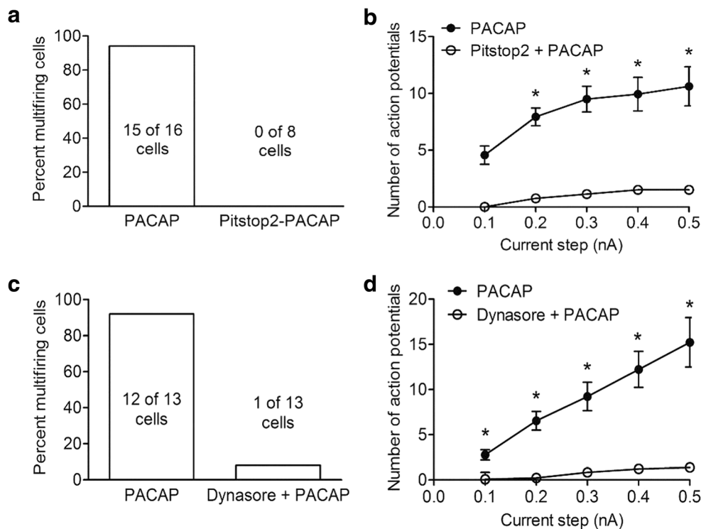
Fig. 3 Pretreatment with Pitstop2 or dynasore suppresses the PACAP-induced increase in excitability. A The percentage of cells exhibiting multiple firing when exposed to PACAP alone ( n = 16 ) was significantly greater than that exposed to PACAP after pretreatment with 15 \mu\text{M} Pitstop2 ( n = 8 ; Fisher's exact test, P < 0.0001 ). B Averaged excitability curves show that Pitstop2 greatly suppressed the PACAP-induced increase in excitability. Asterisks indicate the number of action potentials generated at each current step was significantly greater in PACAP ( n = 16 ) than in PACAP and Pitstop2 ( n = 8 ; unpaired t test, P < 0.0001 for steps 0.2–0.5 nA). C The percentage of cells exhibiting
