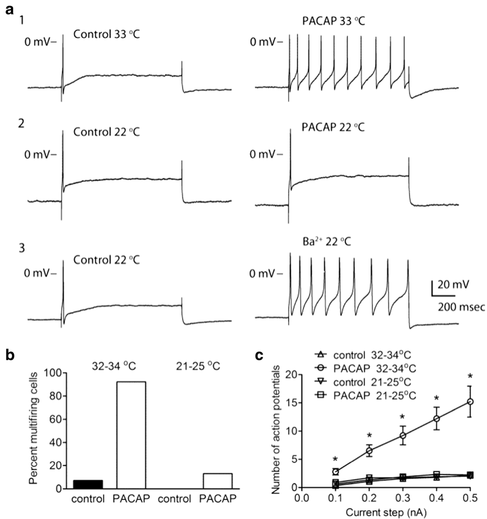
Fig. 2 PACAP-induced increase in excitability is temperature sensitive. A Recordings from different cells showed that 20 nM PACAP increased excitability when the bath solution was 33 °C (A1), but not when the bath temperature was 22 °C (A2). The recording in (A3) demonstrated that the addition of 1 mM BaCl 2 (Ba 2+ ) increased excitability at 22 °C. In all three recordings, the cells exhibited a phasic firing pattern prior to the addition of PACAP (A1, A2) or barium (A3). The firing pattern shifted to multiple firing in (A1, A3), but not in (A2). The amplitude of the 1-s depolarizing current pulse was 0.3 nA in each experiment. B The percentage of cells exhibiting multiple firing in 20 nM PACAP was significantly greater when the temperature was 32–34 °C ( n = 13 cells) than when the bath temperature was 21–25 °C ( n = 23 cells; Fisher’s exact test, P < 0.0001; Also, at 32–34 °C: control ( n = 28) vs. PACAP ( n = 13), significantly
