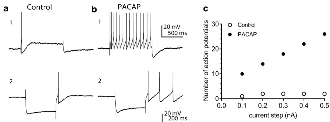
Fig. 1 PACAP can enhance excitability, rectification, and a hyperpolarization-induced rebound depolarization in guinea pig cardiac neurons. Indicators (A1, B1) illustrate the 20-nM PACAP-induced shift from phasic to multiple action potential generation. Prior to PACAP application, a 1 s, 0.2 nA depolarizing constant current pulse elicited 1 action potential. During exposure to PACAP, the number of action potentials generated by the same depolarizing current pulse increased markedly. Indicators (A2, B2) show that PACAP also increased the
