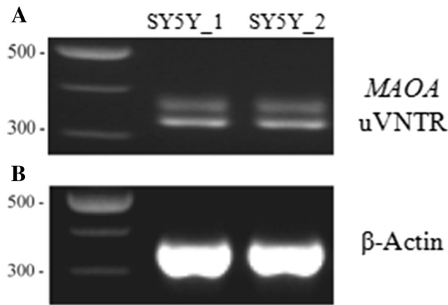
Fig. 2 Monoamine oxidase A ( MAOA ) expression in SH-SY5Y cell line. a PCR assay using uVNTR primer set demonstrating expression of MAOA mRNA under basal conditions. b Expression of \beta -Actin in the same SH-SY5Y samples
