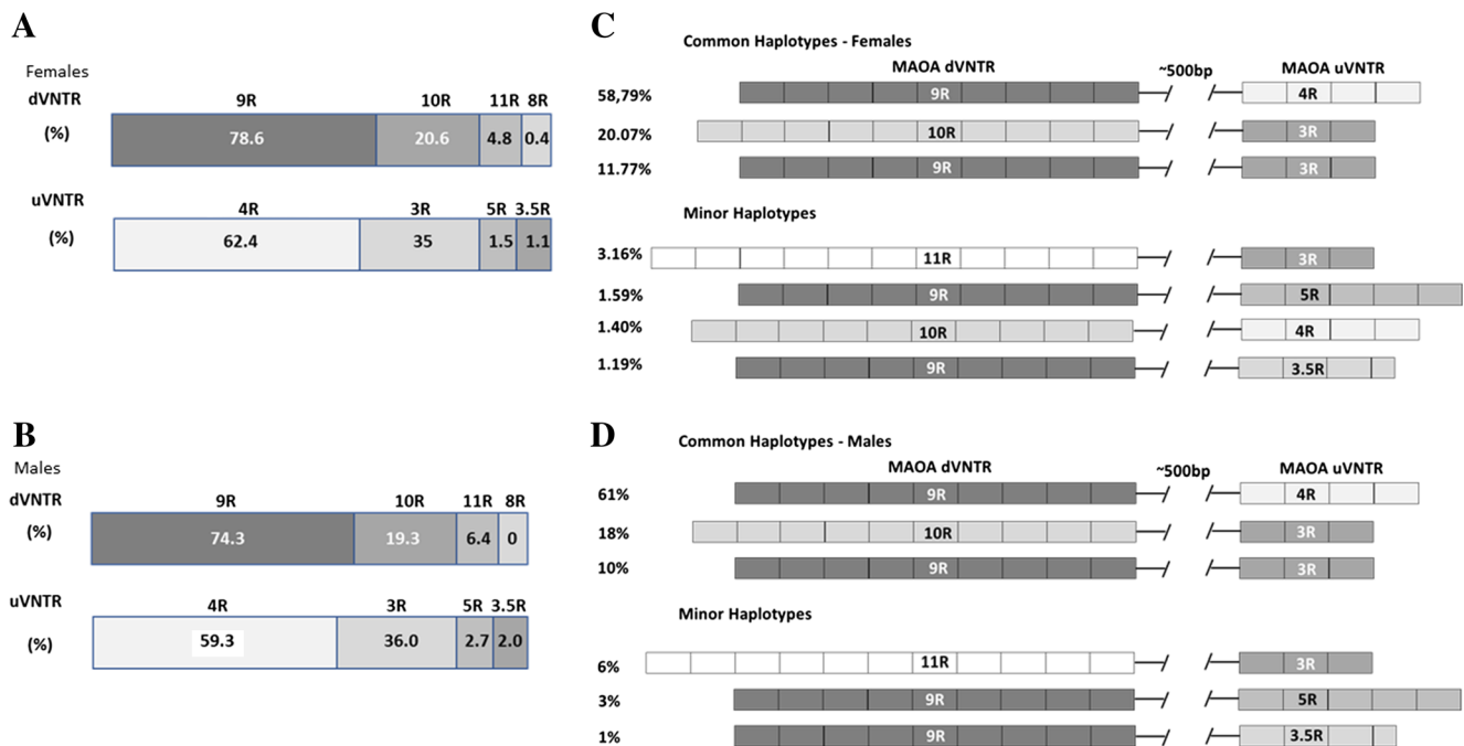
Fig. 6 Allele frequencies ( a, b ) and haplotype distribution ( c, d ) in the Wirral child health and development study (WCHADS, n = 283 ). Assuming a multiallelic system for both markers, the haplotype constructs, frequency, and distribution are illustrated above ( n = 262 ). Haplotypes were initially inferred from males and then the Midas
