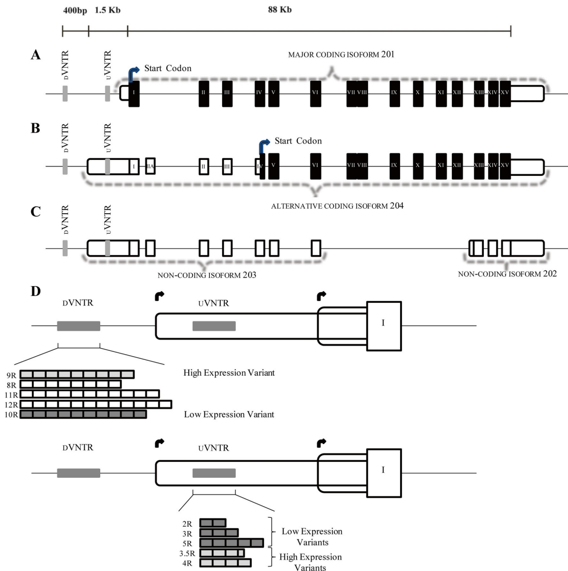
Fig. 1 Monoamine oxidase A ( MAOA ) isoforms. Graphic representation of the MAOA gene as reported in UCSC genome browser Hg38 and the most recent version of the Hg19. White rounded boxes represent 5' and 3' UTRs, and black boxes the translated exons. Curved black arrows indicate the translational start sites. Gray bars are the dVNTR and the uVNTR from left to right respectively. a Major MAOA isoform; NCBI accession number: BC008064 (Version BC008064.2), Ensembl version 201. b MAOA secondary isoform; NCBI accession number: AK293926 (Version AK293926.1), Ensembl version 204. c Untranslated processed
