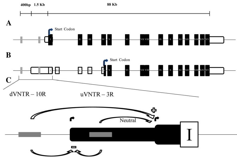
Fig. 7 Regulation model for monoamine oxidase A ( MAOA ) expression by the u- and dVNTRs. Graphic representation of the MAOA promoter region and the regulatory effect exerted by the u- and dVNTRs on the two MAOA isoforms. White box represent exon I, gray bars represent MAOA dVNTR and uVNTR from left to right respectively, and overlapped black boxes represent 5'UTRs of the two isoforms. Curved black lines represent the transcriptional start sites (TSSs) for the two MAOA isoforms
