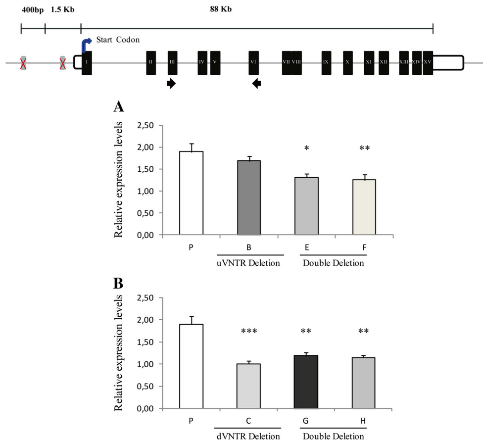
Fig. 4 Total monoamine oxidase A ( MAOA ) expression in HAP1 cell lines under basal conditions—single deletion clones and related double KO clones. Illustrated at the top is the MAOA gene as reported in UCSC genome browser Hg38 and the most recent version of the Hg19. White boxes represent 5' and 3' untranslated regions (UTRs), black boxes the exons, and black straight arrows show the forward and reverse primer sites, respectively. a P is the parental cell line, B single uVNTR deletion
