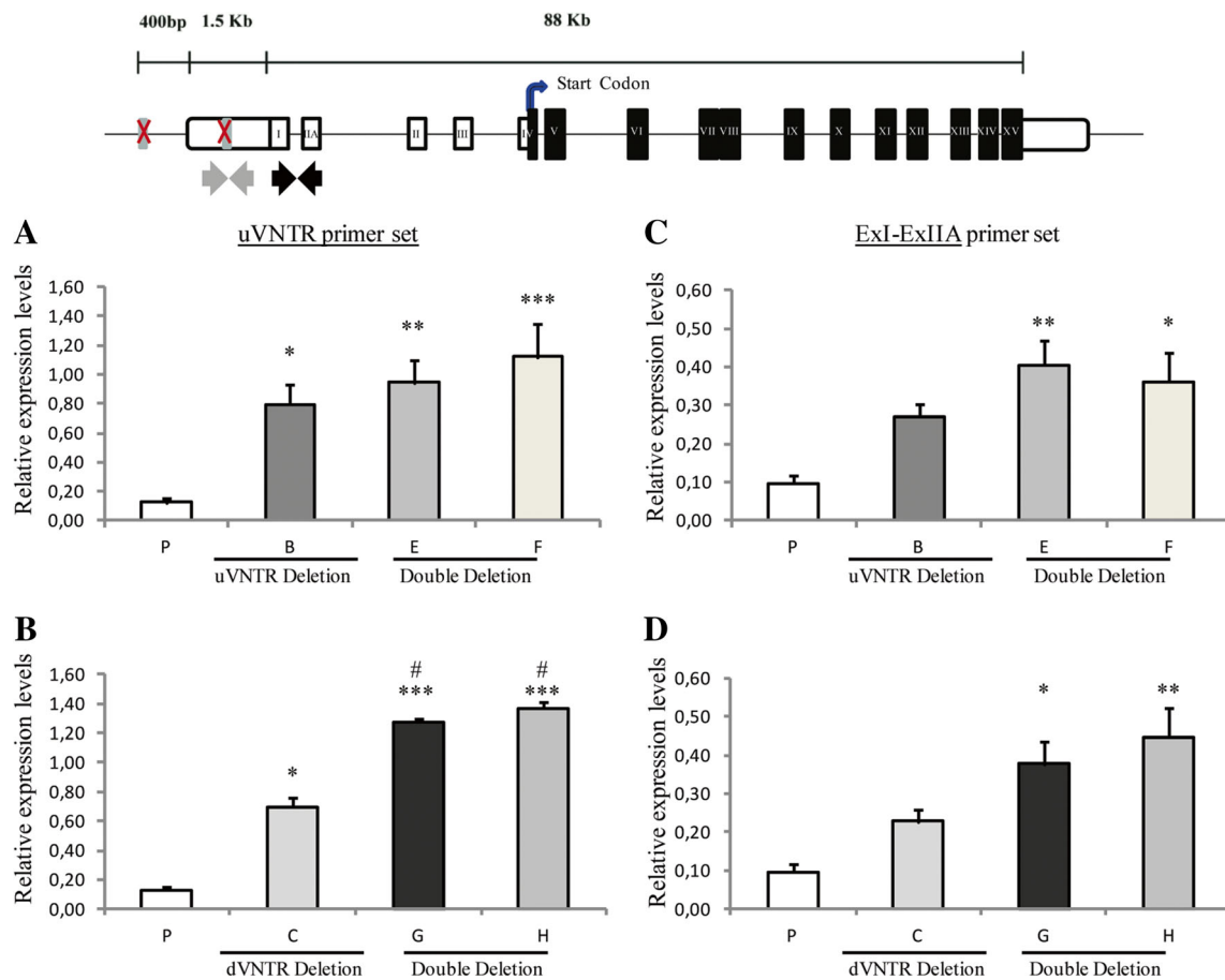
Fig. 5 Monoamine oxidase A ( MAOA ) minor isoform expression in HAP1 cell lines under basal condition—single deletion clones and related double KO clones. At the top illustration of MAOA gene as reported in UCSC genome browser Hg38 and the most recent version of the Hg19. White boxes represent 5' and 3' untranslated regions (UTRs), black boxes the exons. Curved black arrow indicates the translational start site. Black and gray straight arrows show the forward and reverse binding sites for the primers used in analysis. P is the parental cell line, B single uVNTR deletion clone, E(du_B5), and F (du_F3) are the MAOA VNTR double KO clones generated from clone B, C single
