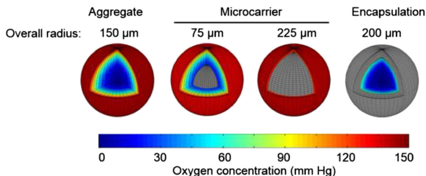
Fig. 3 Comparison of the profile of O_2 in different 3D culture modes, i.e. hPSCs cultured as aggregates, on microcarrier or after encapsulation in alginate beads. Profiles were generated using a reaction–diffusion model assuming Michaelis–Menten kinetics for O_2 consumption by cells and pertinent parameters for diffusion in 1 % alginate matrices [156, 157]. Color regions represent the O_2 profile of hPSCs and gray regions indicate
