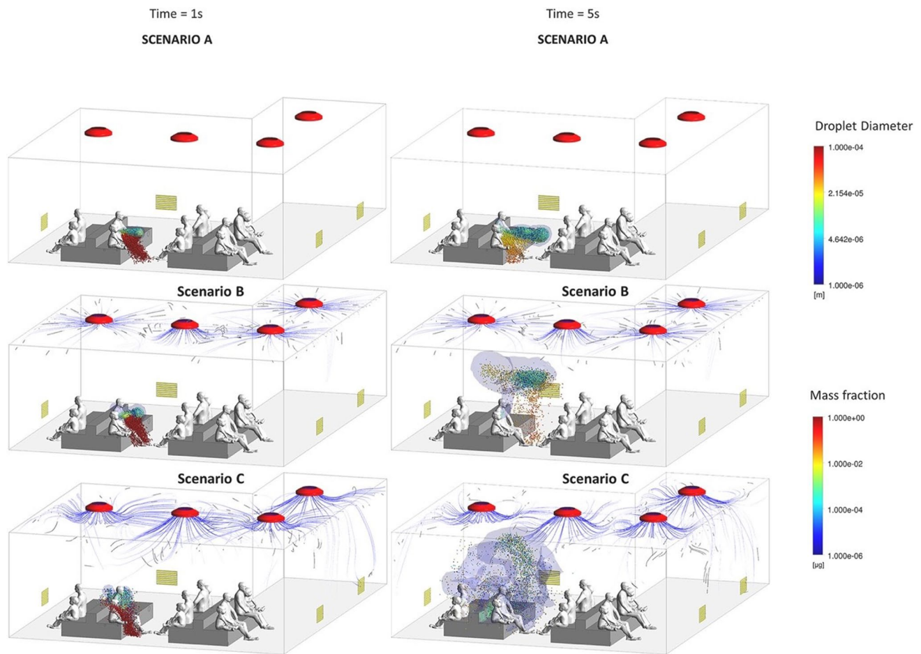
Fig. 13 Prospective view of the Scenarios A, B and C at t=1 s (left) and 5 s (right). The spheres represent the droplets coloured by the diameter size (top right legend). The contaminated air is represented
