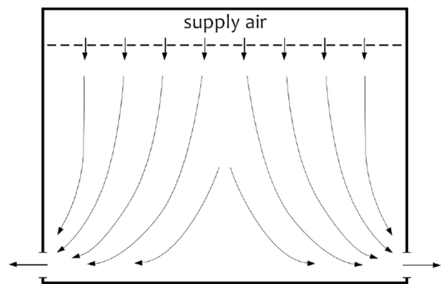
Fig. 6 Displacement downward ventilation pattern
