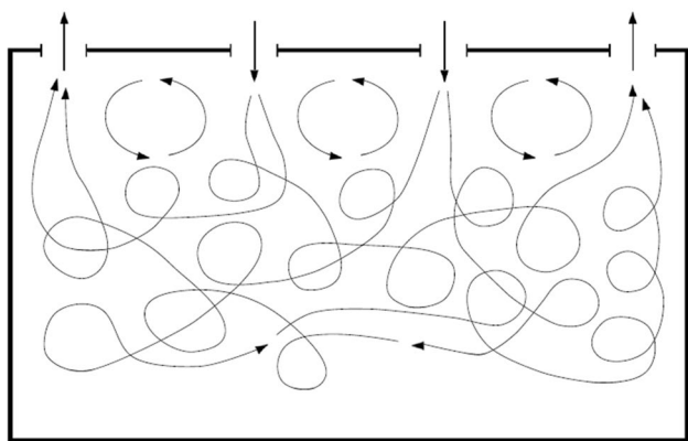
Fig. 8 Mixed ventilation (MV) pattern
