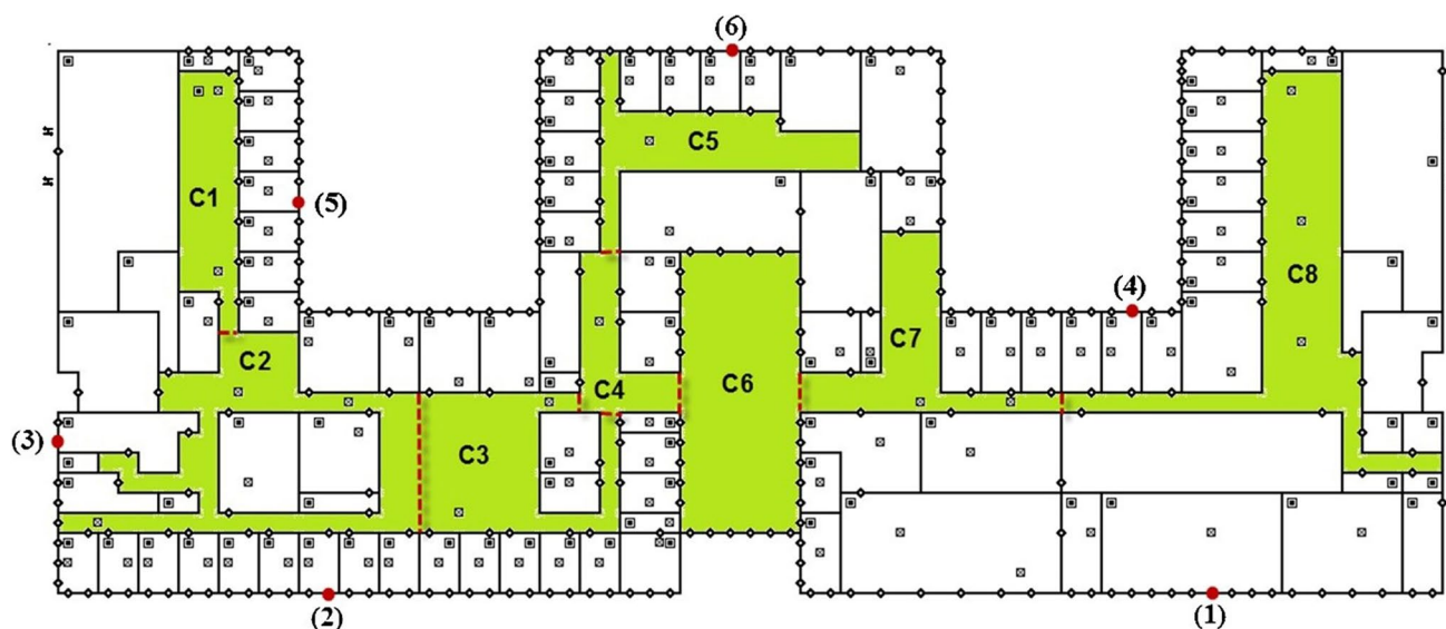
Fig. 10 Building layout produced by CONTAM according to available HVAC data Reproduced from Reference (Argyropoulos et al. 2017a, b) with permission from Elsevier
