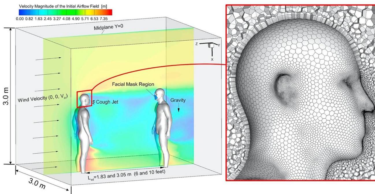
Fig. 12 Schematic of the computational domain with two virtual humans and the hybrid mesh details. Reproduced from Ref (Feng et al. 2020a, b) with permission from Elsevier
