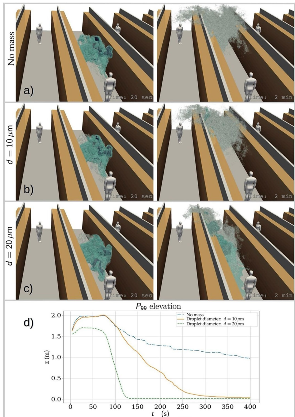
Fig. 11 Visualisations demonstrating the effect of particle size (and mass) on the modelled spreading of the cough-released aerosol cloud. For better sense of scale, bystanders are placed 8 m from the coughing person. Instantaneous views on the state of the cloud are shown for realisations where the particles have a no mass, b 1000 \text{ kg m}^{-3} density and 10\text{-}\mu\text{m} diameter and c 1000 \text{ kg m}^{-3} density and 20\text{-}\mu\text{m} diameter. Images on the left column are at t=20 \text{ s} and on the right column at t=120 \text{ s} . Below, d presents the time evolution of the mean elevation of the 99th percentile concentration highlighting the different descent rates. Droplets in these size scales have \tau_{\text{evap}} < 1 \text{ s} and they would become aerosol-like droplet nuclei very rapidly. Reproduced from Reference (Vuorinen et al. 2020) with permission from Elsevier
