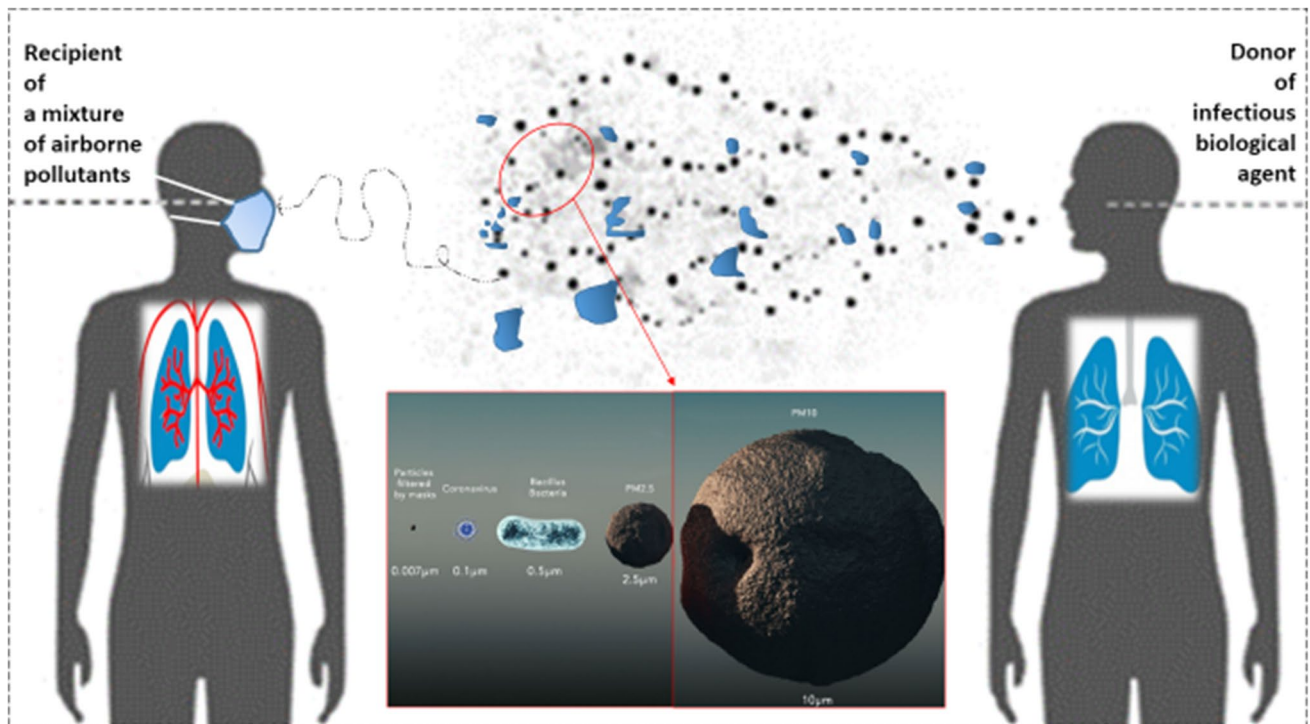
Fig. 1 Schematic representation of a variety of biological (infectious) and chemical agents' transmission between humans via the airborne route
