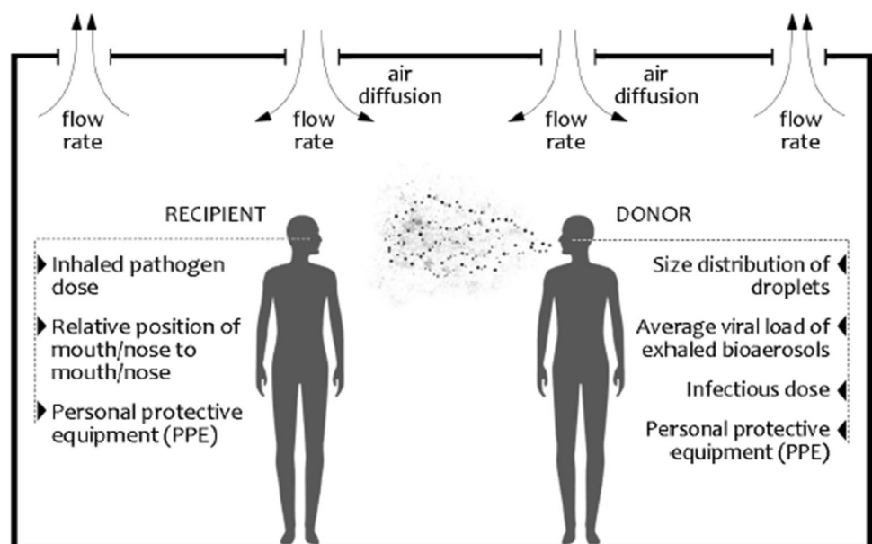
Fig. 4 A donor-recipient model of transmission of respiratory pathogens within droplets
