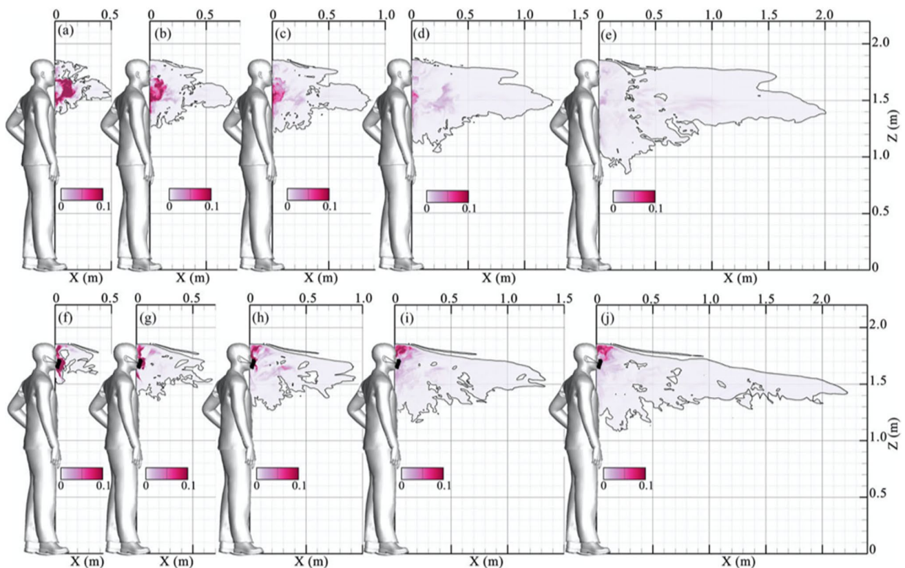
Fig. 14 Simulated evolution of the 10- \mu\text{m} saliva particulate concentration (volume fraction) after the cough under outdoor conditions (mild breeze) without (top) and with (bottom) the facial mask. [(a) and (f)], [(b) and (g)], [(c) and (h)], [(d) and (i)] and [(e) and (j)] show the simulated saliva particulate concentration fields after 0.24 s,
