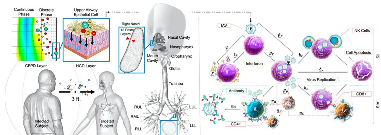
Fig. 15 The framework of the multiscale CFPD-HCD model for the human-to-human IAV infection with a subject-specific airway geometry. The description of the HCD model is given in the ‘The human respiratory system’ section of the original paper (Haghnegahdar et al. 2019a). The detail of the final polyhedral-core mesh is provided at the
