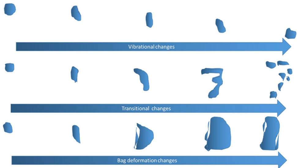
Fig. 2 Schematic representation of the vibrational, transitional and bag deformation shape changes of water droplets traveling in air adapted from (Soni et al. 2020)
