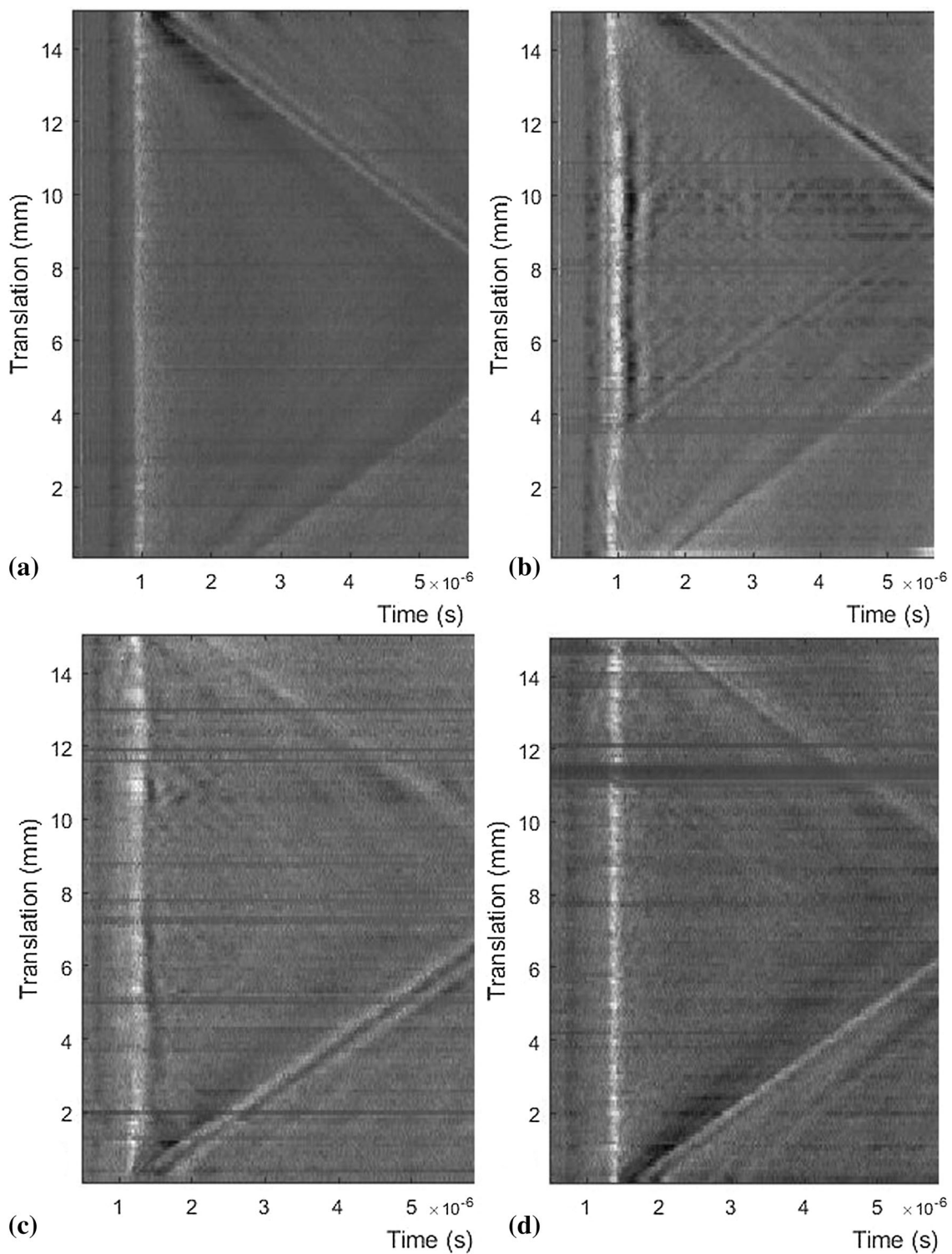
Fig. 2. B-scans comparing (a) bulk material (Sample 1—scan path 1), (b) increased hatch spacing (Sample 1—scan path 2), (c) undermelting conditions (Sample 3—scan path 2), and (d) overmelting conditions (Sample 4—scan path 2).
