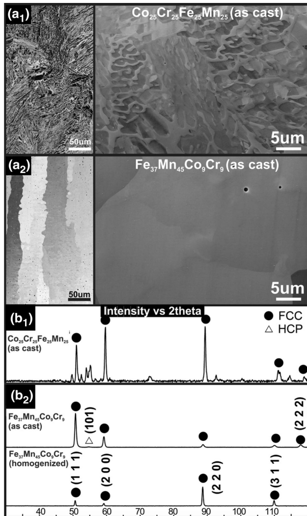
Fig. 2. (a) Light microscopy and (b) XRD-based characterization of the four-component, (b1) \text{Co}_{25}\text{Cr}_{25}\text{Fe}_{25}\text{Mn}_{25} and (b2) \text{Fe}_{37}\text{Mn}_{45}\text{Co}_9\text{Cr}_9 alloys (as cast and homogenized).
