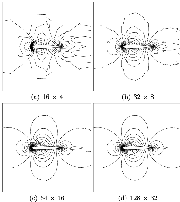
Fig. 54 Inviscid subsonic flow around a NACA0012 airfoil: Mach number isolines with isoparametric FE and p = 1
