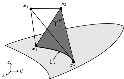
Fig. 14 Curved tetrahedral elements with an edge on the NURBS boundary
