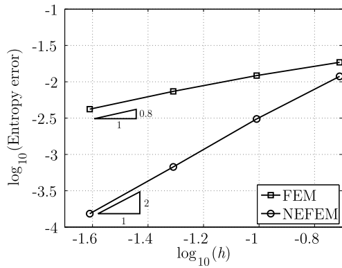
Fig. 52 Inviscid subsonic flow around a circle: h -convergence of the entropy error for isoparametric FEs and NEFEM ( p = 1 )
