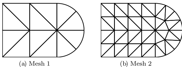
Fig. 34 Coarse meshes for the second-order elliptic problem. Nested remeshing is used for refinement
