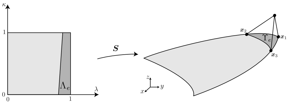
Fig. 13 Curved tetrahedral face on a singular NURBS boundary with a singular point, leading to a quadrilateral \Lambda_e in the parametric space
