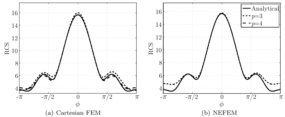
Fig. 73 Scattering by a PEC sphere of diameter \lambda : RCS comparison for increasing p and for the horizontal polarization
