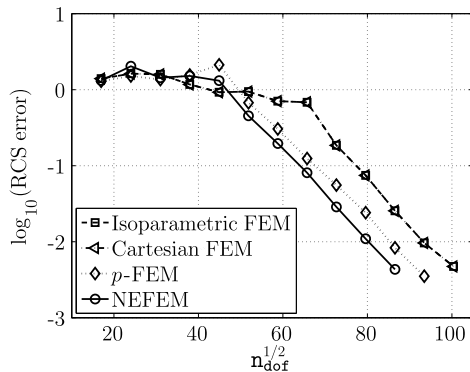
Fig. 66 Scattering by a PEC cylinder of diameter 4\lambda : p -convergence comparison of several curved FEs
