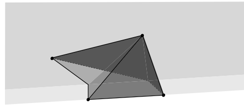
Fig. 90 Detailed view of a NEFEM element containing an edge singularity in its boundary face
