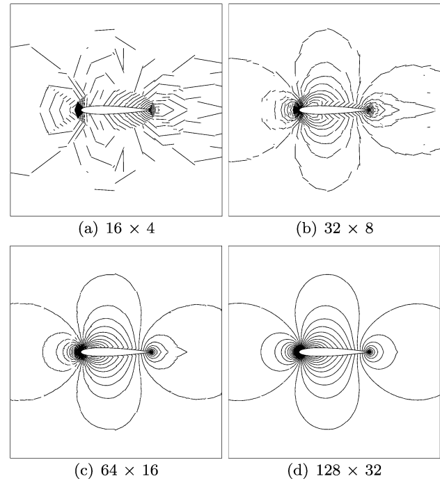
Fig. 55 Inviscid subsonic flow around a NACA0012 airfoil: Mach number isolines with NEFEM and p = 1
