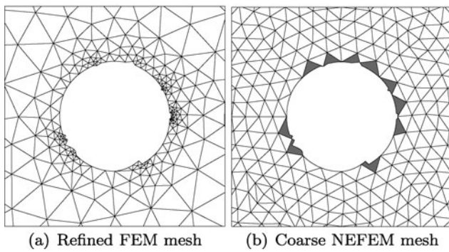
Fig. 84 Scattering by an irregular circular cylinder of diameter 4\lambda : detail of a standard FE mesh refined towards the small geometric details, and a coarse NEFEM mesh with elements containing corner geometric singularities
