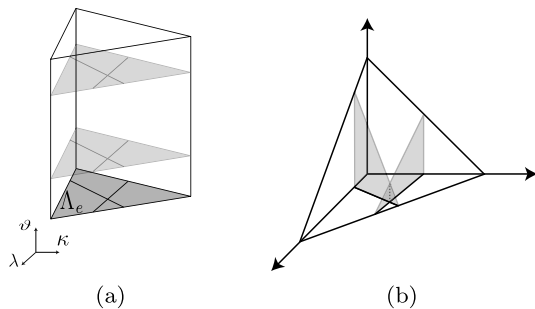
Fig. 33 Subdivisions to design a numerical quadrature taking into account changes of NURBS definition. (a) On the prism \Lambda_e \times [0, 1] for 3D NEFEM and (b) on the reference tetrahedron for 3D p -FEM
