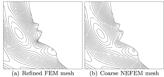
Fig. 86 Scattering by an irregular circular cylinder of diameter 4\lambda : detail of the H_3 field
