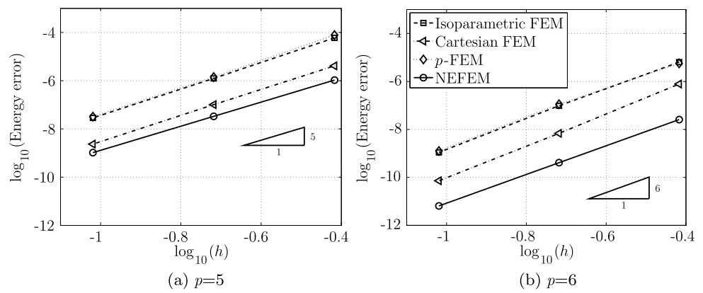
Fig. 36 Second-order elliptic problem: h -convergence in the energy norm
