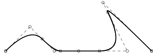
Fig. 2 NURBS curve (solid line), control points (denoted by \circ ), control polygon (dashed line) and breakpoints (denoted by \square )
