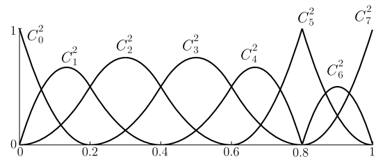
Fig. 1 B-spline basis functions for the knot vector (1)
