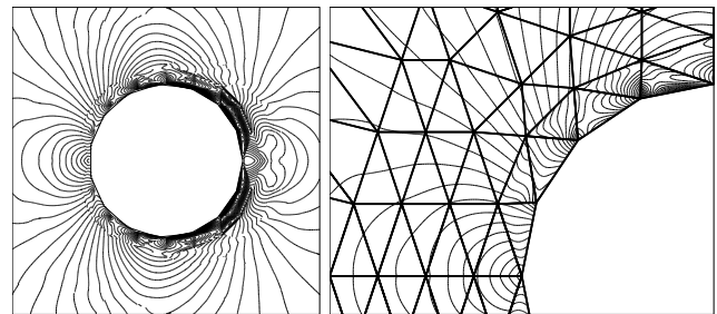
Fig. 59 Inviscid subsonic flow around a circle: subparametric FE solution using straight-sided elements and high-order approximation of the solution ( p = 4 )
