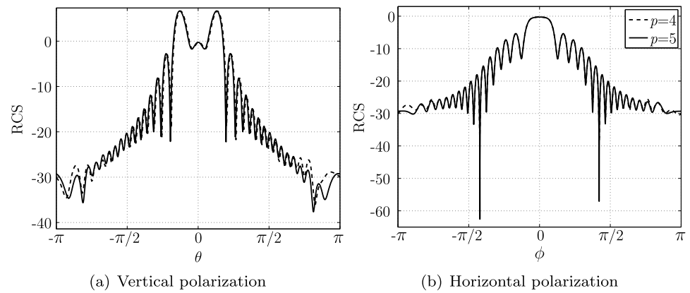
Fig. 81 Scattering by a PEC NASA almond of characteristic length 8\lambda : RCS for a NEFEM solution with p = 5
