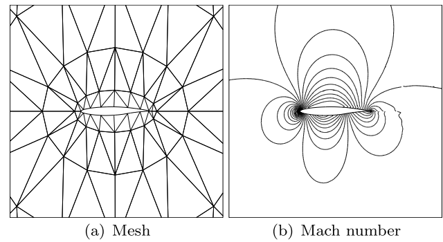
Fig. 62 Inviscid subsonic flow around a RAE2822 airfoil: coarse mesh and Mach number isolines for NEFEM and p = 8
