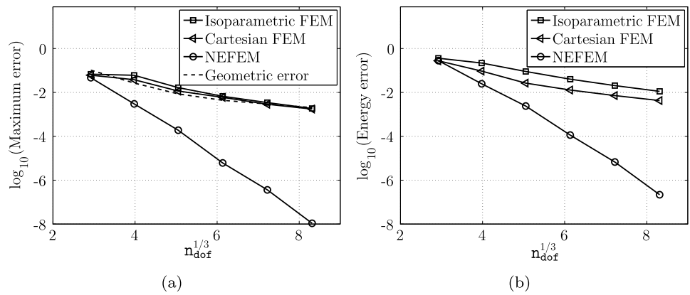
Fig. 43 p -convergence comparison for the second-order elliptic problem. The polynomial degree of the approximation is uniformly increased from p = 2 and the error is measured (a) in the maximum norm and (b) in the energy norm
