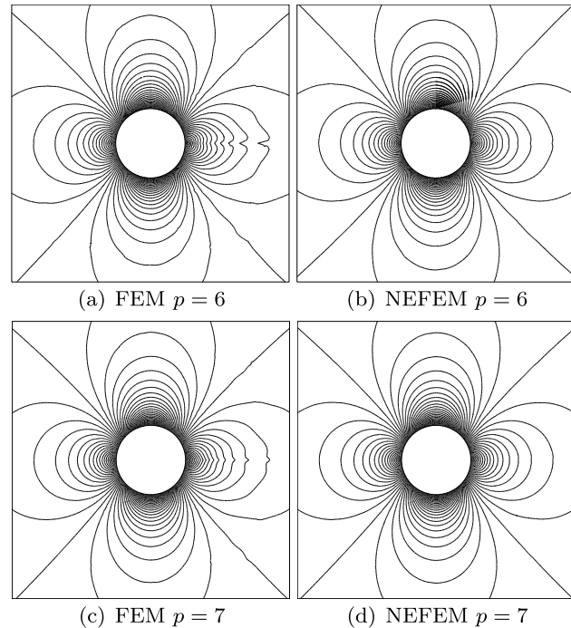
Fig. 61 Inviscid subsonic flow around a circle: Mach number distribution in the coarse mesh shown in Fig. 60 with isoparametric FE and NEFEM and high-order approximations
