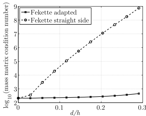
Fig. 21 Condition number of the elemental mass matrix as a function of d/h
