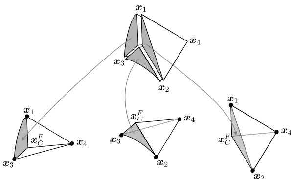
Fig. 25 Splitting used for numerical integration in an element with two edges defined by different NURBS (no new degrees of freedom are introduced)
