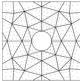
Fig. 60 Inviscid subsonic flow around a circle: coarse mesh and Fekete nodal distribution for p = 6
