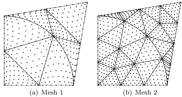
Fig. 45 Two triangular meshes with interior curved edges and Fekette nodal distributions for a degree of approximation p = 8
