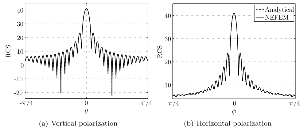
Fig. 79 Scattering by a PEC sphere of diameter 20\lambda : RCS for a NEFEM solution with p = 4 in the range [-\pi/4, \pi/4]
