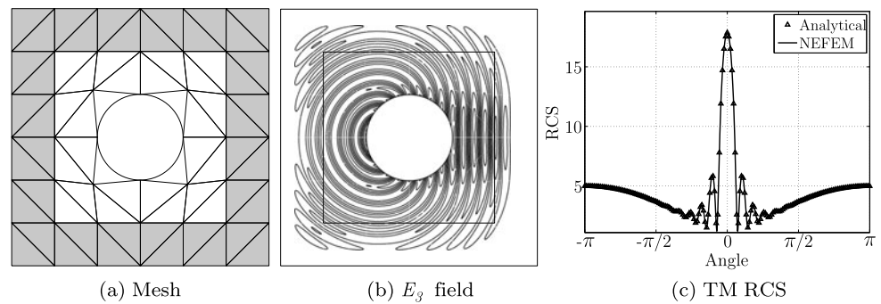
Fig. 65 Scattering by a PEC cylinder of diameter 4\lambda
