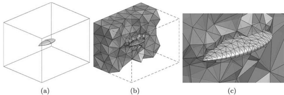
Fig. 8 (a) Domain with part of the boundary defined by curved NURBS surfaces corresponding to the NASA almond, (b) cut through an unstructured tetrahedral mesh with the surface triangular mesh on the almond, and (c) detail of the mesh near the almond
