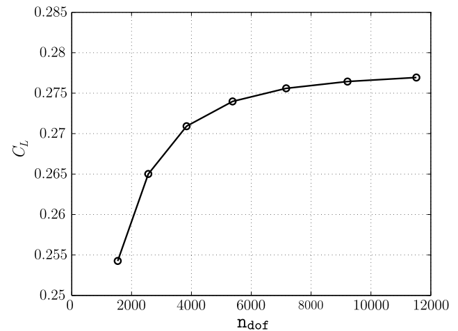
Fig. 63 Inviscid subsonic flow around a RAE2822 airfoil: lift coefficient convergence for increasing p in the mesh of Fig. 62(a)
