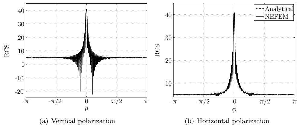
Fig. 78 Scattering by a PEC sphere of diameter 20\lambda : RCS for a NEFEM solution with p = 4
