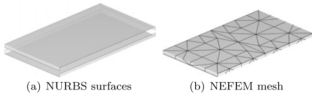
Fig. 89 Scattering by a PEC thin plate: NURBS surfaces (separated for visualization) and NEFEM coarse mesh with elements containing edge singularities
