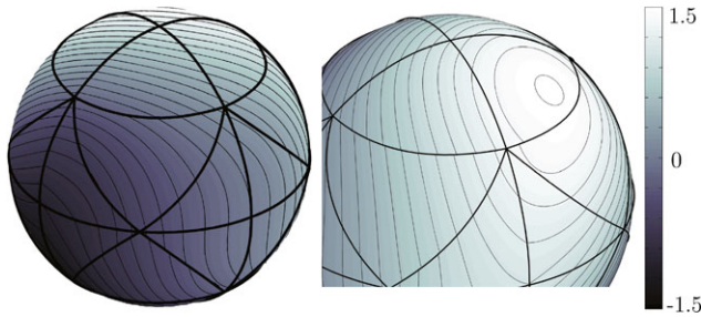
Fig. 47 Solution of the Poisson problem in a sphere and detail of the solution showing a small discontinuity across curved boundary edges
