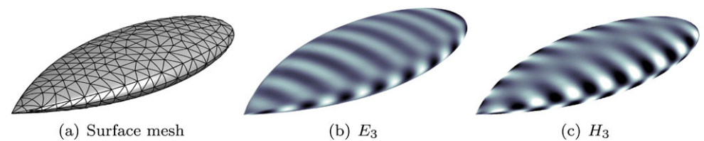
Fig. 80 Scattering by a PEC NASA almond of characteristic length 8\lambda : surface mesh and two components of the scattered field for a NEFEM solution with p = 5
