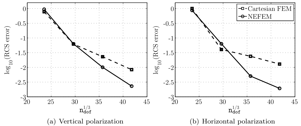
Fig. 74 Scattering by a PEC sphere of diameter \lambda : p -convergence comparison of the RCS error
