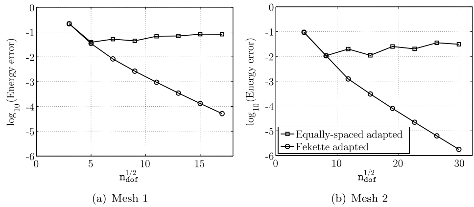
Fig. 46 p -convergence of the error in the energy norm for different nodal distributions on the meshes of Fig. 45
