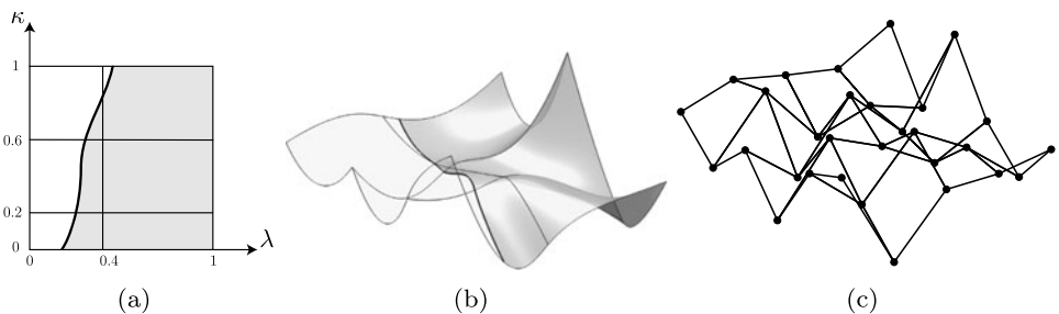
Fig. 6 (a) Parametric space trimmed by the thick curve, (b) trimmed NURBS surface with knot lines and the thick curve used to trim the initial surface of Fig. 5, and (c) control net
