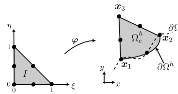
Fig. 28 Isoparametric mapping between the reference element I , with local coordinates \xi , and an approximation of the physical subdomain in Cartesian coordinates x , namely \Omega_e^h = \varphi(I)
