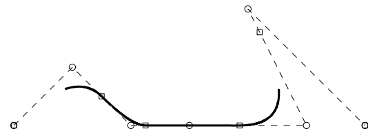
Fig. 3 Trimmed NURBS curve with \lambda \in [0.05, 0.75] (solid line), control points (denoted by \circ ), control polygon (dashed line) and breakpoints (denoted by \square )
