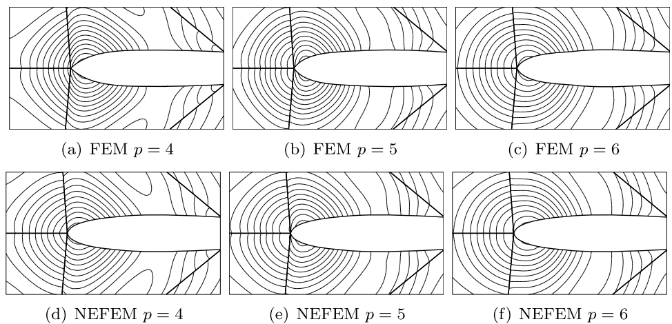
Fig. 69 Scattering by a PEC NACA0012 airfoil of chord length 2\lambda : detailed view of the transverse scattered field near the leading edge for isoparametric FE and NEFEM increasing p
