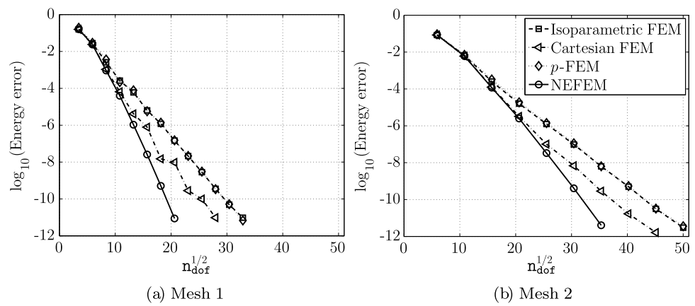
Fig. 38 Second-order elliptic problem: p -convergence in the energy norm for the computational meshes represented in Fig. 34
