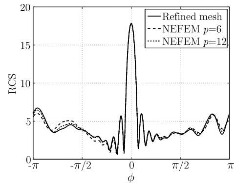
Fig. 87 Scattering by an irregular circular cylinder of diameter 4\lambda : RCS comparison
