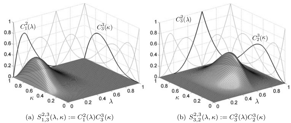
Fig. 4 Example of 2D B-spline basis functions
