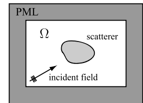
Fig. 64 Schematic of an electromagnetic scattering problem with a PML surrounding the computational domain
