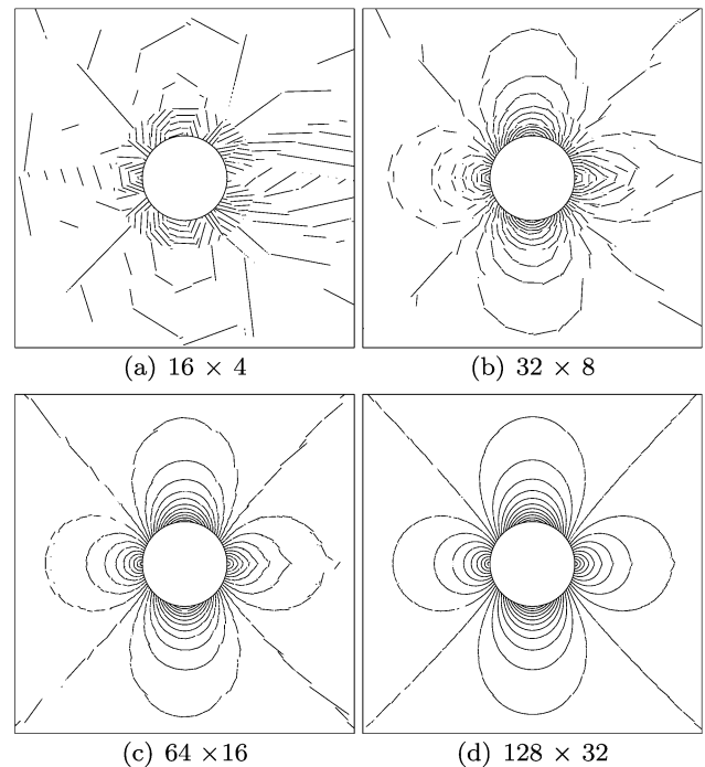
Fig. 50 Inviscid subsonic flow around a circle: Mach number isolines with NEFEM and p = 1
