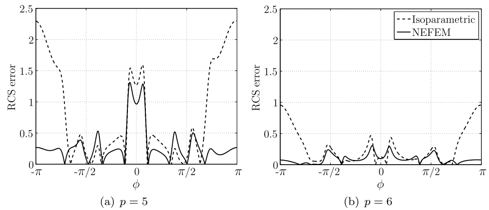
Fig. 70 Scattering by a PEC NACA0012 airfoil of chord length 2\lambda : RCS error comparison for isoparametric FEM and NEFEM
