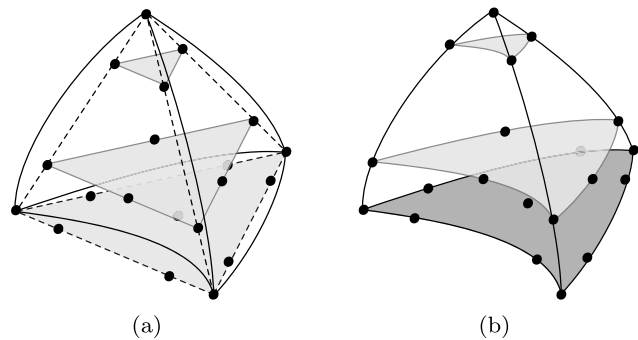
Fig. 19 Fekette nodal distribution for p = 3 (a) defined using the (imaginary) tetrahedral with planar faces, and (b) adapted to the curved geometry
