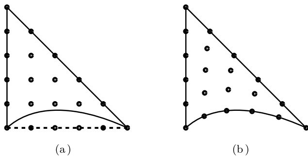
Fig. 15 Equally-spaced nodal distribution for p = 5 (a) defined using the (imaginary) triangle with planar faces, and (b) adapted to the curved geometry
