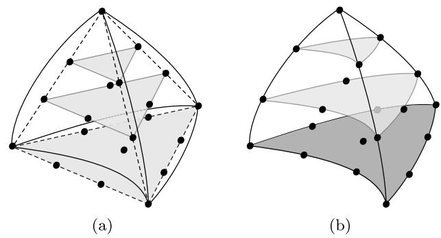
Fig. 16 Equally-spaced nodal distribution for p = 3 (a) defined using the (imaginary) tetrahedral with planar faces, and (b) adapted to the curved geometry
