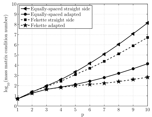
Fig. 17 Condition number of the mass matrix as a function of the interpolation degree ( p )
