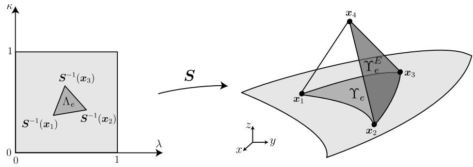
Fig. 11 Parametrization of a curved tetrahedral element with a face on the NURBS boundary, showing a face \Gamma_e on the NURBS boundary, and a face \Gamma_e^E with an edge on the NURBS boundary, \Gamma_e^E
