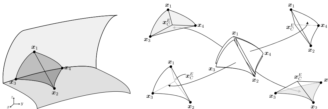
Fig. 26 Splitting used for numerical integration in an element with two faces defined by different NURBS (no new degrees of freedom are introduced)
