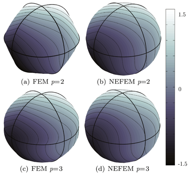
Fig. 42 Second-order elliptic problem: surface plot of Cartesian FEM and NEFEM solutions using quadratic and cubic approximations
