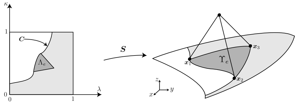
Fig. 12 Curved tetrahedral face on a trimmed NURBS boundary. NURBS surface S is trimmed by NURBS curve C , leading to a curved triangle \Lambda_e in the parametric space
