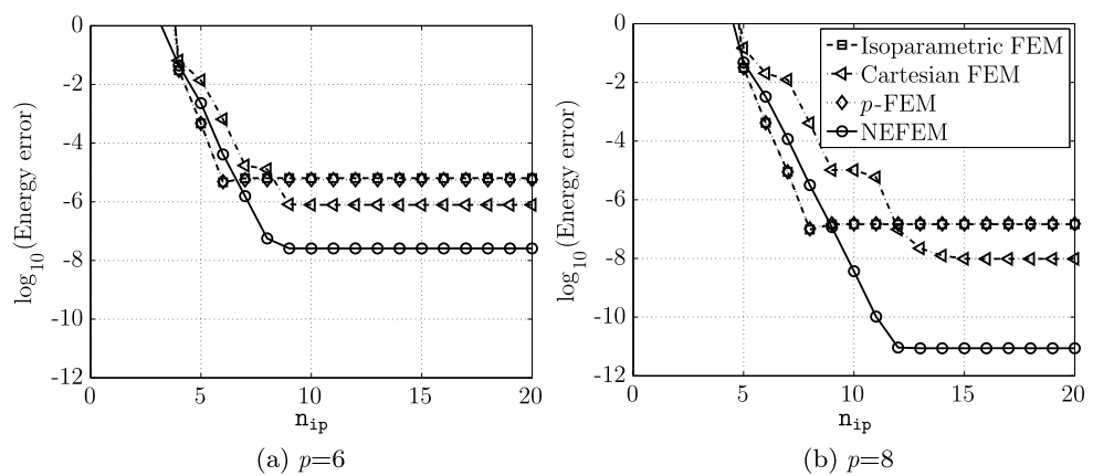
Fig. 39 Second-order elliptic problem: Energy norm of the error as the number of integration points ( n_{ip} ) along the curved boundary edge is increased. Coarse mesh of Fig. 34
