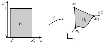
Fig. 10 Parametrization of a curved triangular element with an edge on the NURBS boundary
