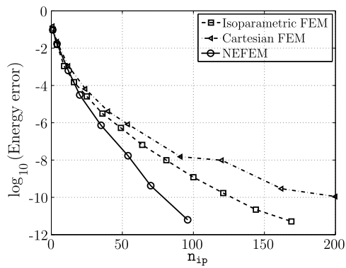
Fig. 40 Second-order elliptic problem: Energy norm of the error vs number of integration points ( n_{ip} ) for interior integrals as p increases using the coarsest mesh in Fig. 34
