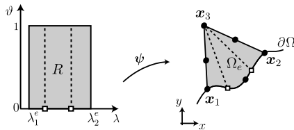
Fig. 32 Numerical integration for 2D NEFEM: subdivision of the rectangle R = [\lambda_1^e, \lambda_2^e] \times [0, 1] to design a numerical quadrature taking into account changes of NURBS parametrization C(\lambda) at points marked with \square
