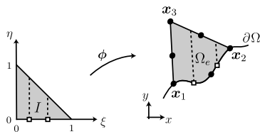
Fig. 31 Numerical integration for 2D p -FEM: subdivision of the reference element I to design a numerical quadrature taking into account changes of NURBS parametrization C(\xi) at points marked with \square
