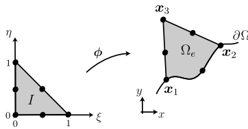
Fig. 29 Exact mapping between the reference element I with local coordinates \xi , and the physical subdomain \Omega_e with Cartesian coordinates x
