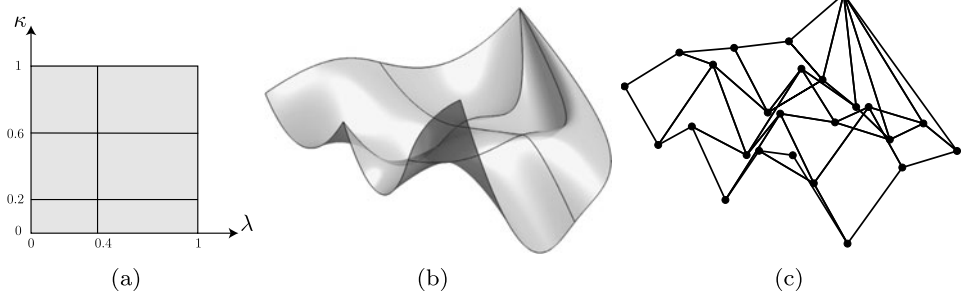
Fig. 7 (a) Parametric space, (b) singular NURBS surface with knot lines, and (c) control net
