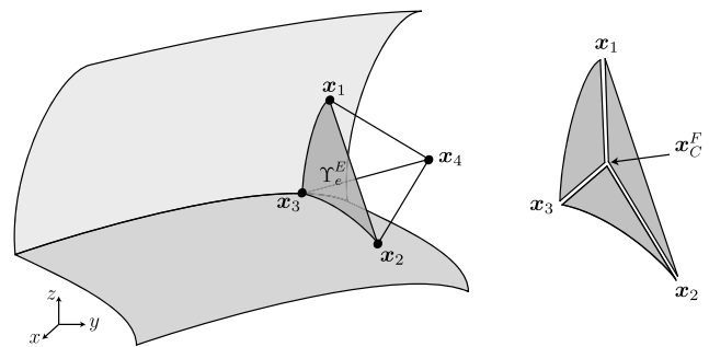
Fig. 23 Tetrahedral element with two edges on different NURBS boundaries, and face splitting used for numerical integration (no new degrees of freedom are introduced)
