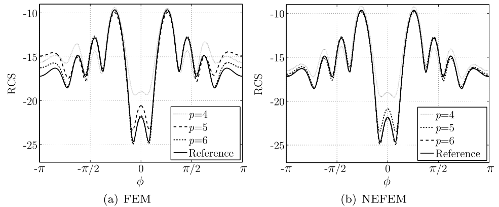
Fig. 68 Scattering by a PEC NACA0012 airfoil of chord length 2\lambda : TE RCS comparison as p increases
