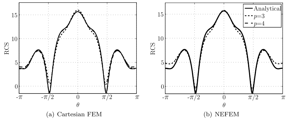
Fig. 72 Scattering by a PEC sphere of diameter \lambda : RCS comparison for increasing p and for the vertical polarization
