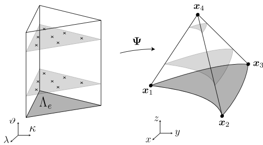
Fig. 27 Transformation from \Lambda_e \times [0, 1] to \Omega_e to perform numerical integration on an element with a face on the NURBS boundary
