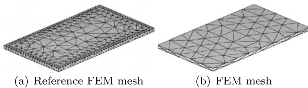
Fig. 88 Scattering by a PEC thin plate: standard FE meshes
