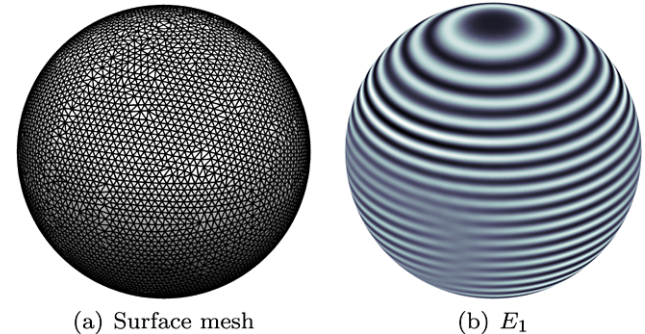
Fig. 77 Scattering by a PEC sphere of diameter 20\lambda
