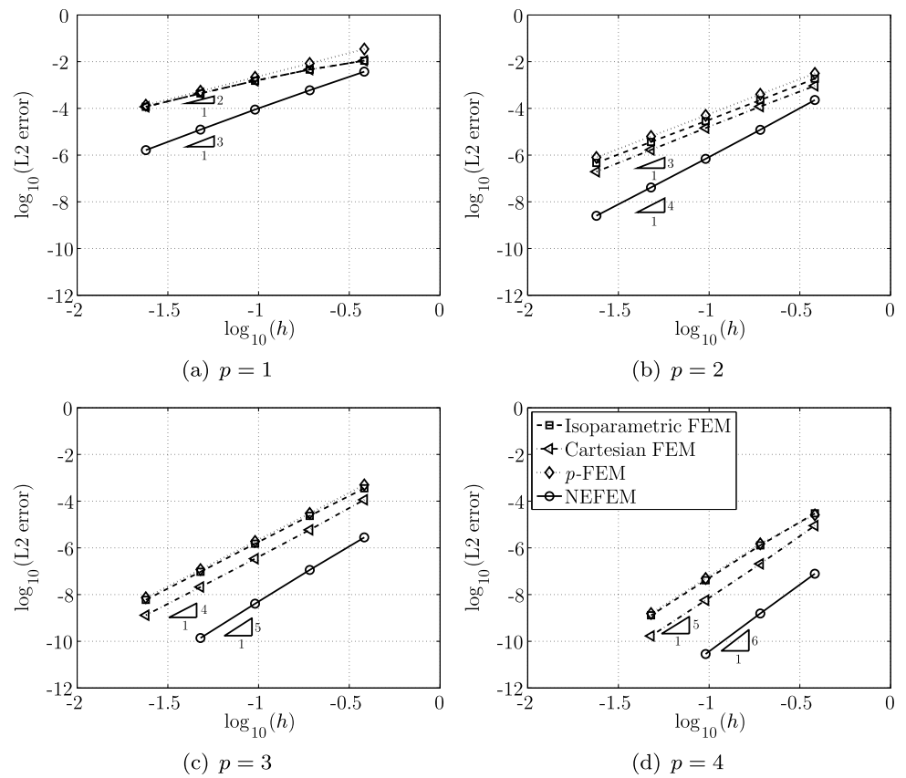
Fig. 37 Second-order elliptic problem: h -convergence in the \mathcal{L}^2(\Gamma_n) norm
