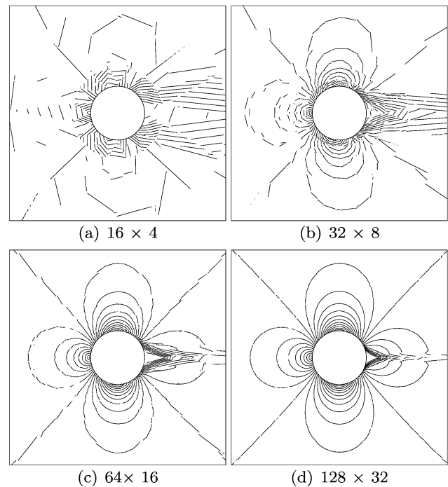
Fig. 49 Inviscid subsonic flow around a circle: Mach number isolines with isoparametric FE and p = 1
