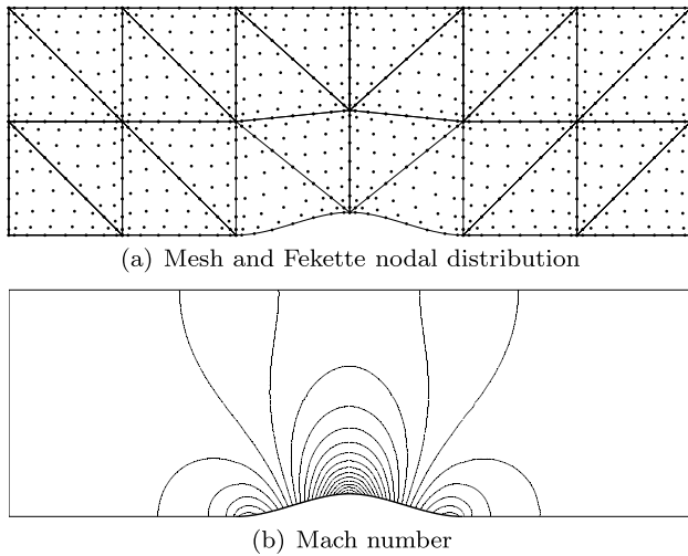
Fig. 57 Inviscid subsonic flow over a bump: (a) Coarse mesh and (b) NEFEM solution with p = 8
