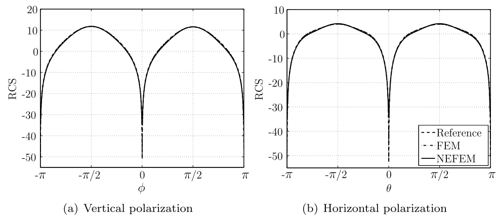
Fig. 91 Scattering by a PEC thin plate: comparison of the RCS computed in the discretizations shown in Figs. 88(a), 88(b) and 89(a)
