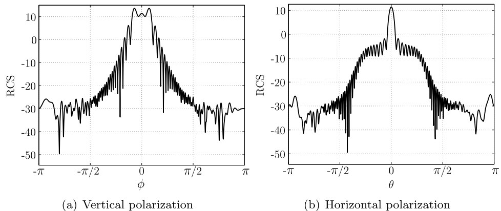
Fig. 83 Scattering by a PEC NASA almond of characteristic length 21\lambda : RCS for a NEFEM solution with p = 4
