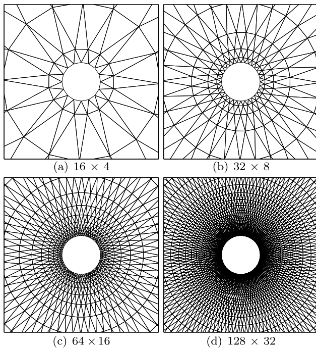
Fig. 48 Inviscid subsonic flow around a circle: detail of O-meshes for low-order computations
