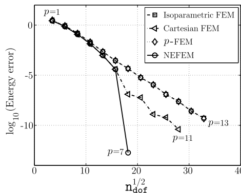
Fig. 35 Poisson problem with polynomial analytical solution: p -convergence in the energy norm in the coarse mesh of Fig. 34
