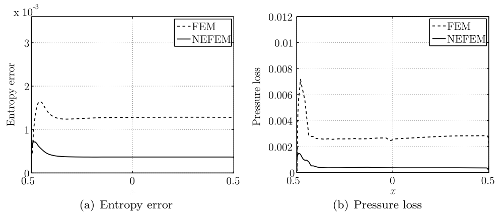
Fig. 56 Inviscid subsonic flow around a NACA0012 airfoil: (a) entropy error and (b) pressure loss in the upper part of the airfoil
