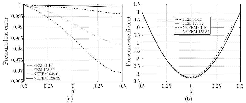
Fig. 51 Inviscid subsonic flow around a circle: (a) Pressure loss distribution and (b) pressure coefficient distribution, at the upper mid of the circle for p = 1
