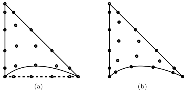
Fig. 18 Fekette nodal distribution for p = 5 (a) defined using the (imaginary) triangle with planar faces, and (b) adapted to the curved geometry
