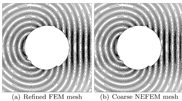
Fig. 85 Scattering by an irregular circular cylinder of diameter 4\lambda : H_3 field computed in the discretizations shown in Fig. 84
