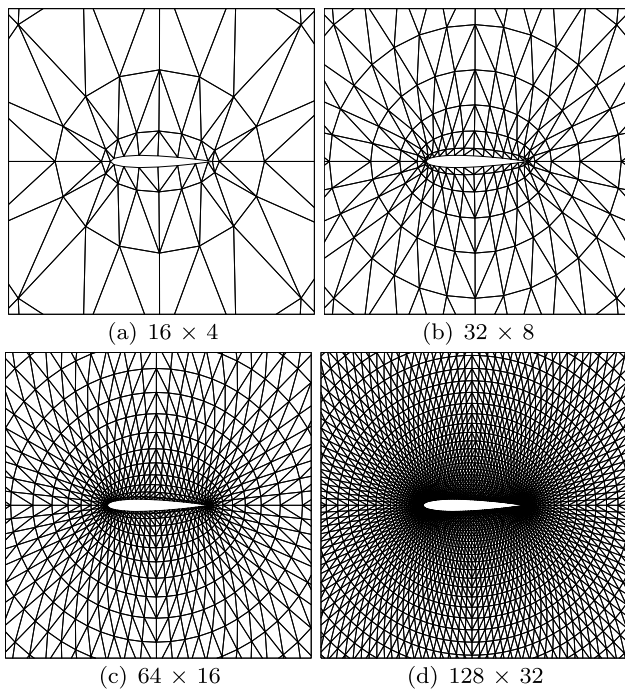
Fig. 53 Inviscid subsonic flow around a NACA0012 airfoil: detail of O-meshes for low-order computations
