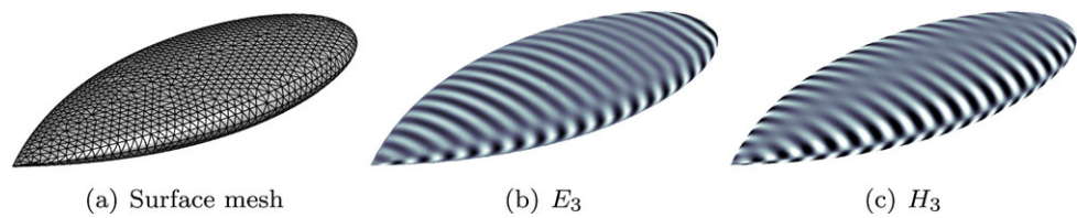
Fig. 82 Scattering by a PEC NASA almond of characteristic length 21\lambda : surface mesh on the almond and two components of the scattered field for a NEFEM solution with p = 3
