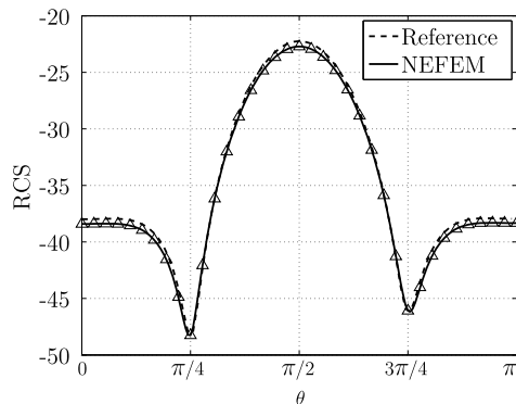
Fig. 76 Scattering by a PEC NASA almond of characteristic length \lambda : monostatic RCS for a NEFEM solution with p = 4 , compared with high-order edge elements of [59]
