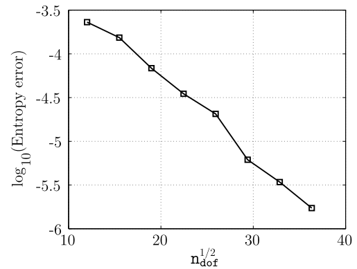
Fig. 58 Inviscid subsonic flow over a bump: p -convergence of the entropy error with NEFEM
