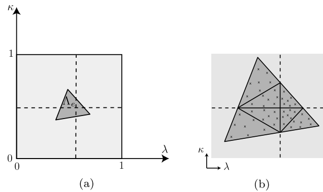
Fig. 24 Definition of a numerical quadrature on A_e for the numerical integration on a curved tetrahedral face with changes of NURBS parametrization along discontinuous lines (knot lines): (a) triangle in the parametric space and (b) detailed view of the composite quadrature
