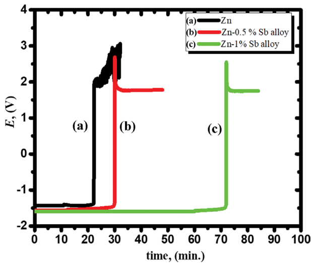
Fig. 2. Relation between anodic polarization potential and time of Zn specimen (a), and its alloys I (b) and II (c) in the concentrated basic electrolyte at 50 \text{ mA cm}^{-2} and 25^\circ \text{C} .
