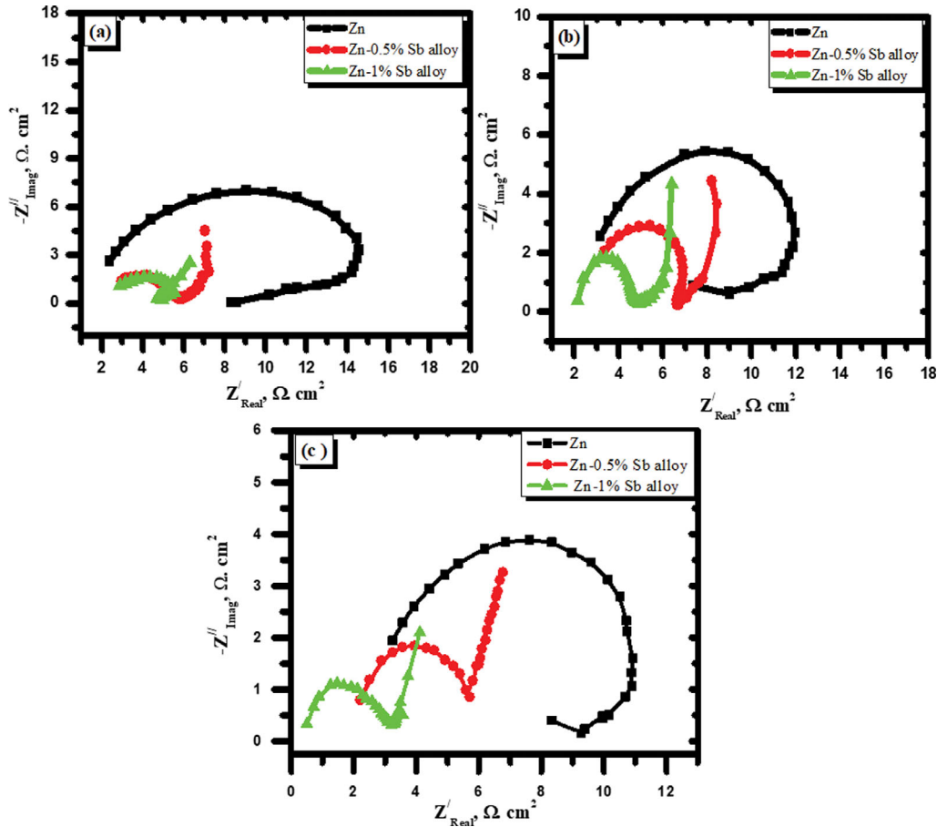
Fig. 7. Comparison between the experimental data of Nyquist plots of the Zn specimen and its alloys I and II in a concentrated alkaline solution of the passive film formed at various positive values of the potential of +0.5 V (a), +0.8 V (b), and +2.0 V (c), at 25 °C.
