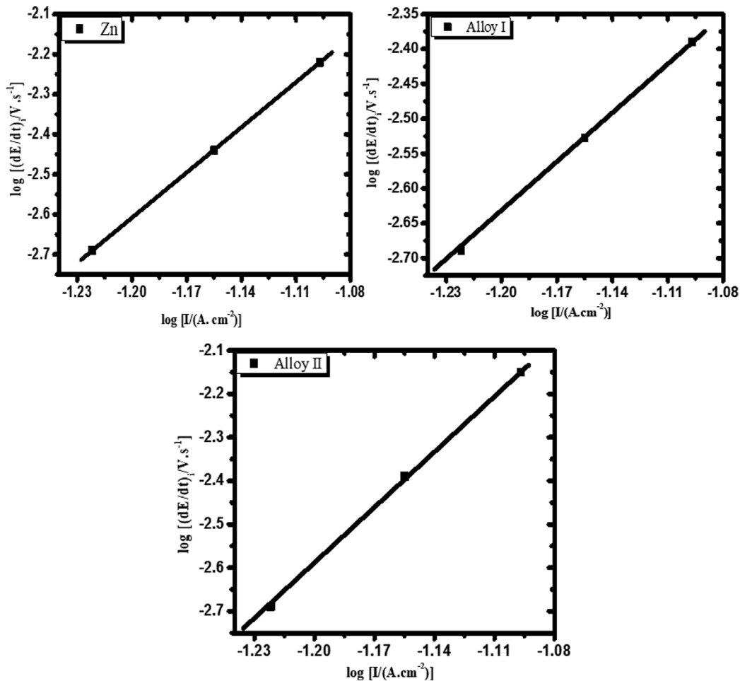
Fig. 5. A logarithmic relationship between the rate of oxide film generation ( dE/dt ); and the imposed current density for Zn specimen (a), alloy I, and II (c) in the concentrated basic solution and at 25 °C.
