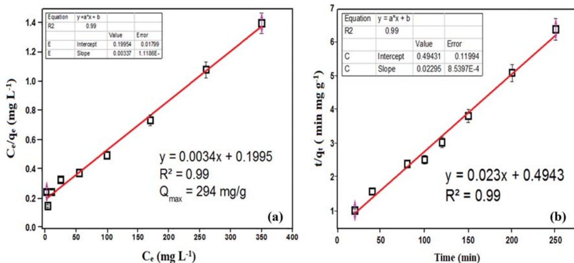
Fig. 8. The plot of (a) Langmuir adsorption isotherm, (b) pseudo-second-order model.
