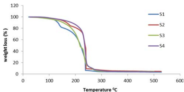
Fig. 4. TG curves of various \text{TiO}_2 samples.
