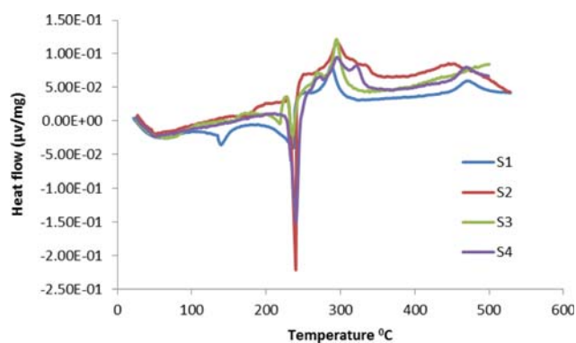
Fig. 5. DSC curves of various \text{TiO}_2 samples.
