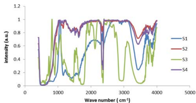
Fig. 6. FT-IR spectra of various \text{TiO}_2 samples.
