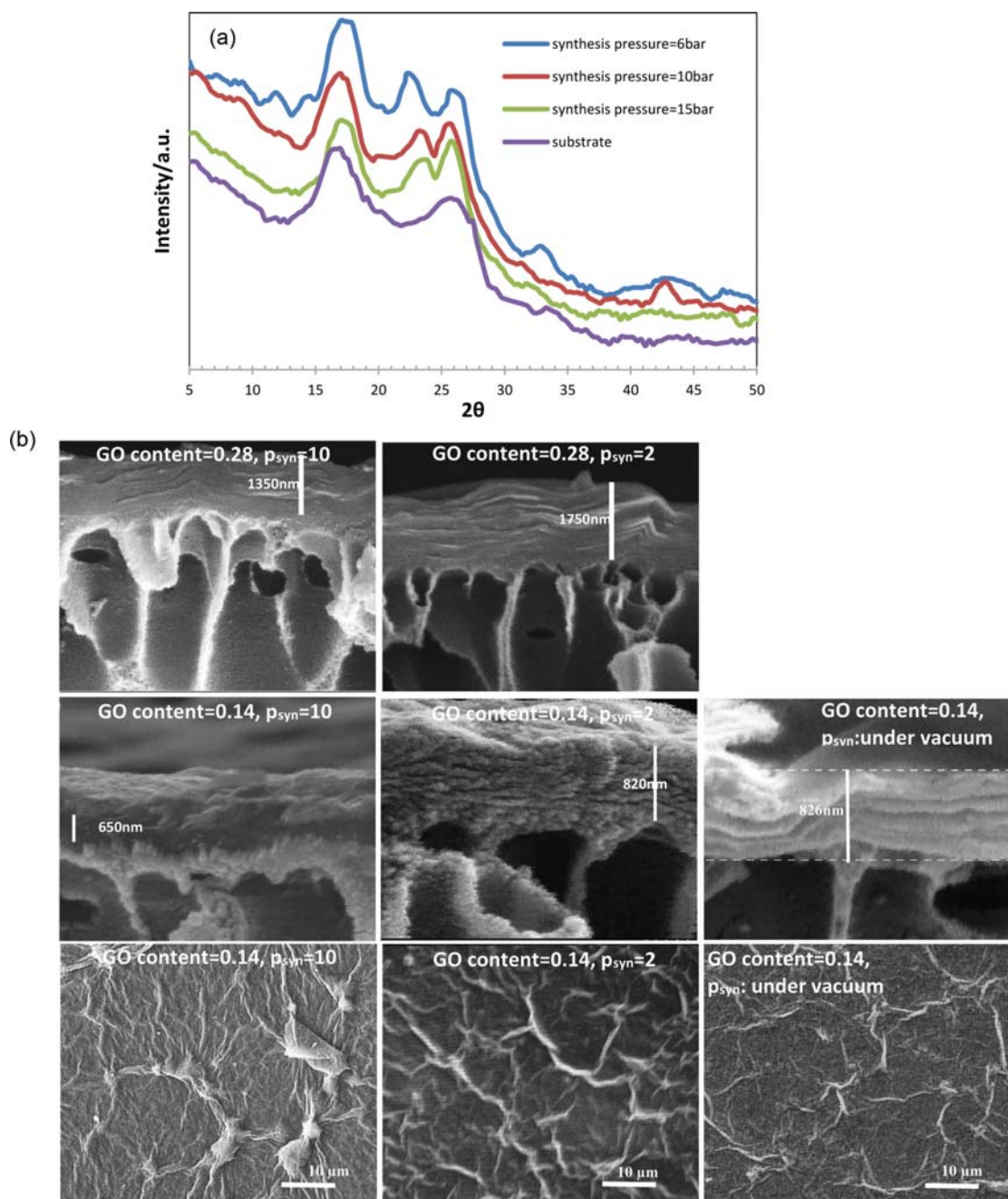
Fig. 9. Effect of synthesis pressure on (a) interlayer spacing of substrate and GO membranes and (b) cross section of 0.28 \text{ mg/cm}^2 GO membrane (upper row), cross-section (middle row) and surface (lower row) of 0.14 \text{ mg/cm}^2 GO membrane. Left to right: p_{\text{syn}}=10, 2 bar and under vacuum.
