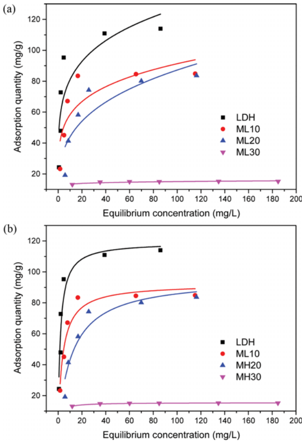
Fig. 8. Adsorption isotherms of ARG dye on LDH and ML. (a) Freundlich isotherm, (b) Langmuir isotherm.
