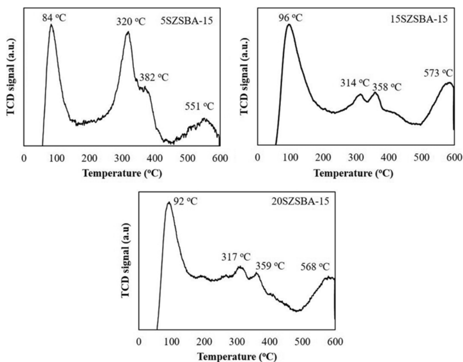
Fig. 7. NH_3 -TPD profiles of 5SZSBA-15, 15SZSBA-15 and 20SZSBA-15 catalysts.
