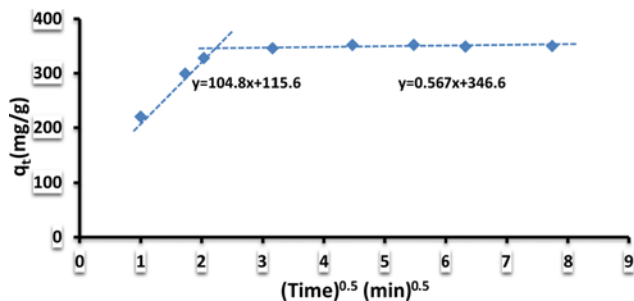
Fig. 13. Intraparticle diffusion of MB by SBA-15.
