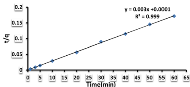
Fig. 12. Pseudo-second order kinetics models.
