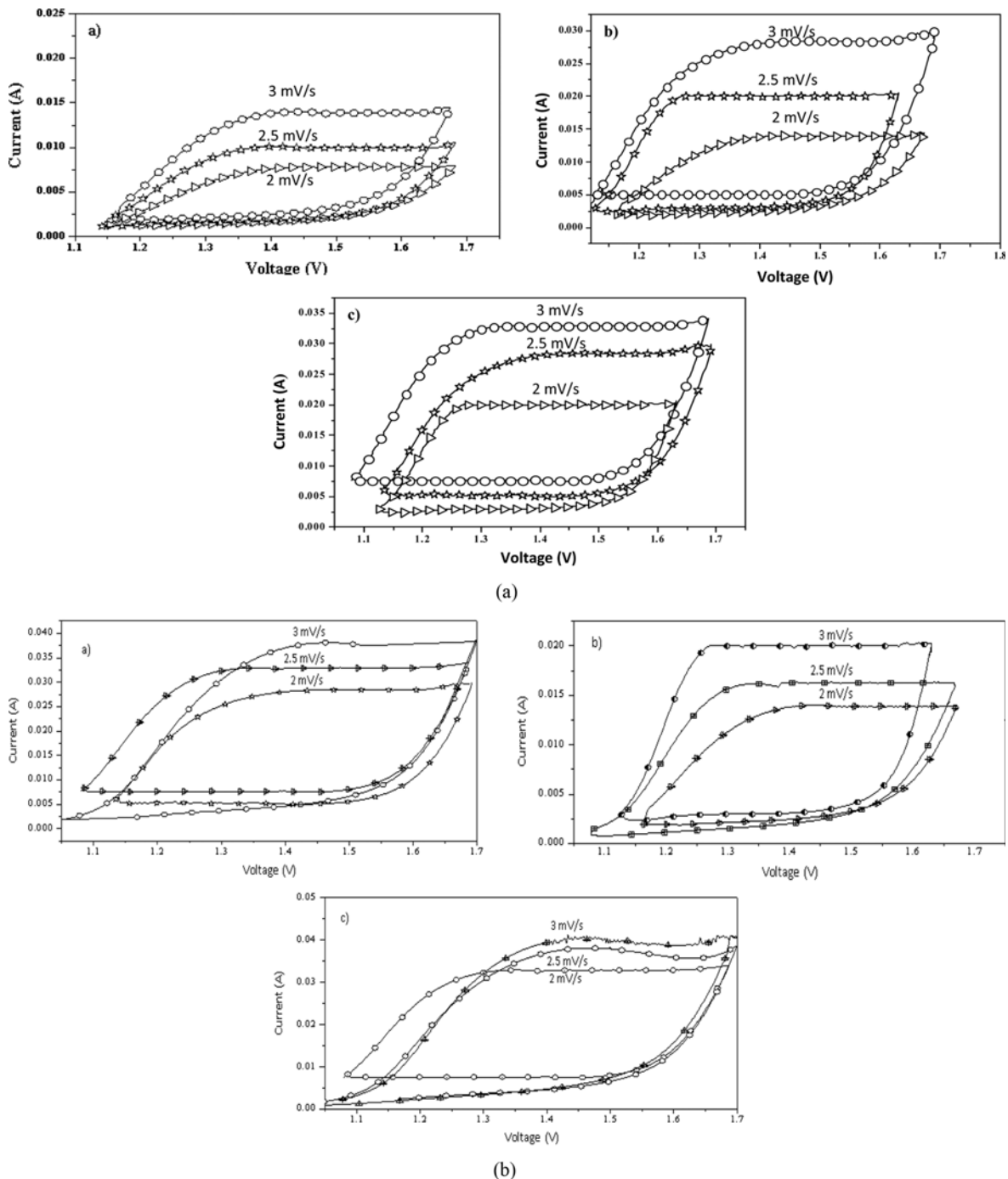
Fig. 4. (a) The cyclic voltammogram of a) SC 600 b) SC 700 and c) SC 800 using 1 M H_2SO_4 as electrolyte at different scan rates. (b) The cyclic voltammogram of a) RS 600 b) RS 700 and c) RS 800 using 1 M H_2SO_4 as electrolyte at different scan rates.
