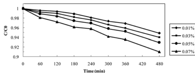
Fig. 8. Variation in relative concentration of silica in nanofluids over time.
