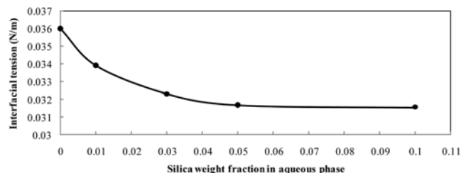
Fig. 1. Interfacial tension for different concentrations of SiO 2 nanoparticles.
