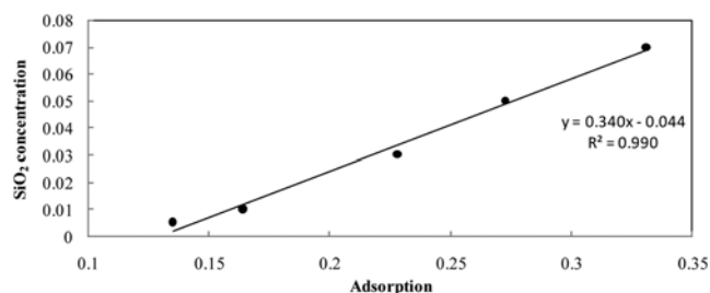
Fig. 7. Calibration curve of silica concentration with corresponding light absorption.
